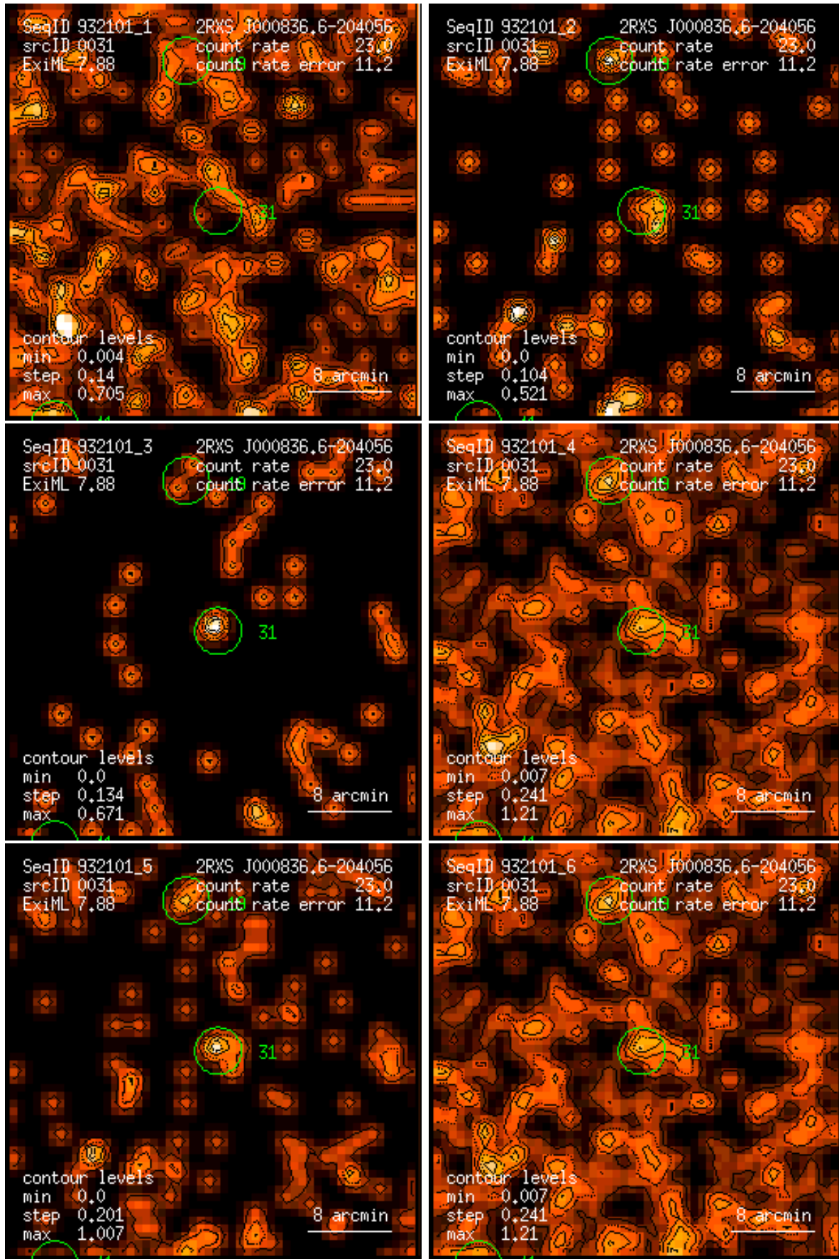
Figure 31: RASS 932101: detection 0031: band rate images, Gaussian filter: (1) PSPC channels 11 – 41, (2) 52 – 90, (3) 91 – 201, (4) 11 – 235, (5) 52 – 201, (6) 11 – 201. Broad band rates in counts/ks. Band rate contour levels in counts/ks/arcmin 2 .
