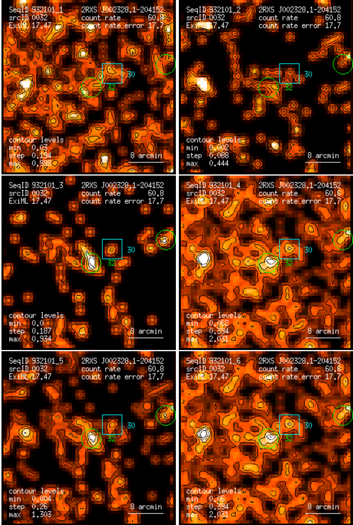
Figure 32: RASS 932101: detection 0032: band rate images, Gaussian filter: (1) PSPC channels 11 – 41, (2) 52 – 90, (3) 91 – 201, (4) 11 – 235, (5) 52 – 201, (6) 11 – 201. Broad band rates in counts/ks. Band rate contour levels in counts/ks/arcmin 2 .
