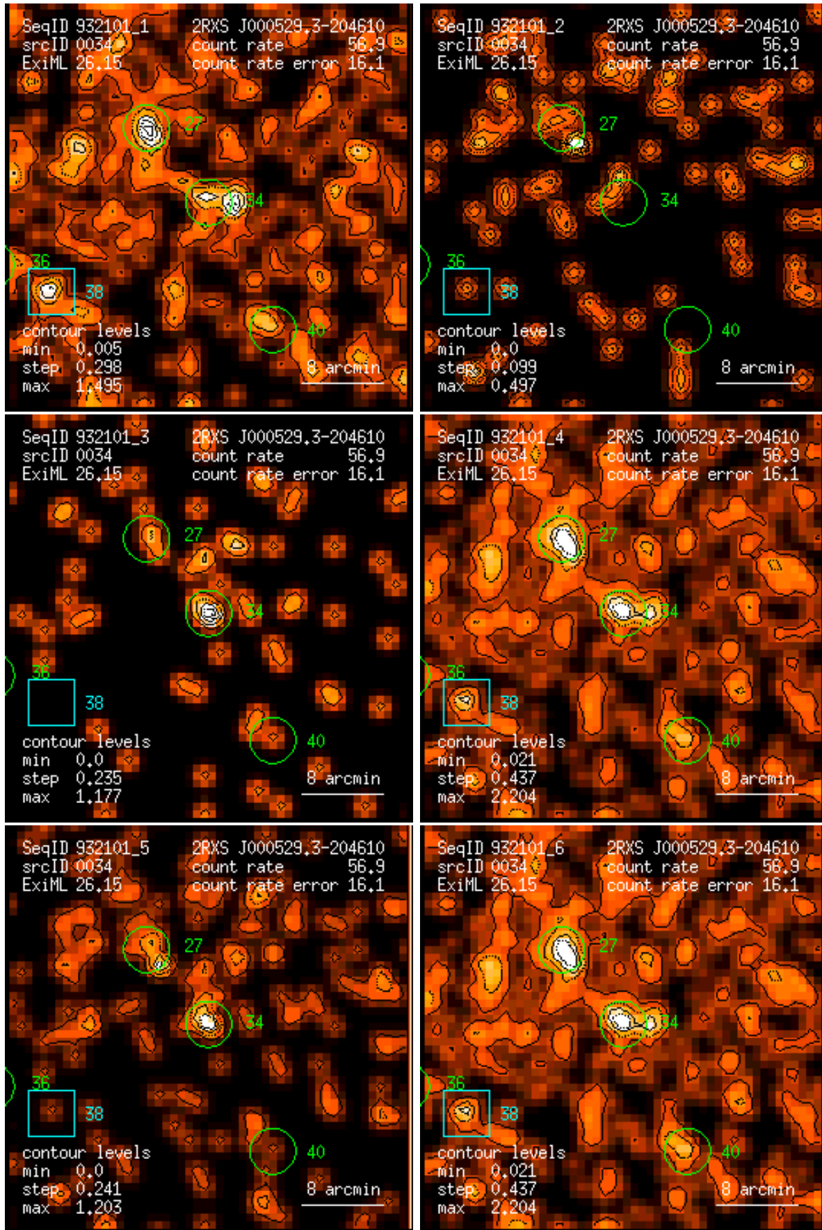
Figure 34: RASS 932101: detection 0034: band rate images, Gaussian filter: (1) PSPC channels 11 – 41, (2) 52 – 90, (3) 91 – 201, (4) 11 – 235, (5) 52 – 201, (6) 11 – 201. Broad band rates in counts/ks. Band rate contour levels in counts/ks/arcmin 2 .
