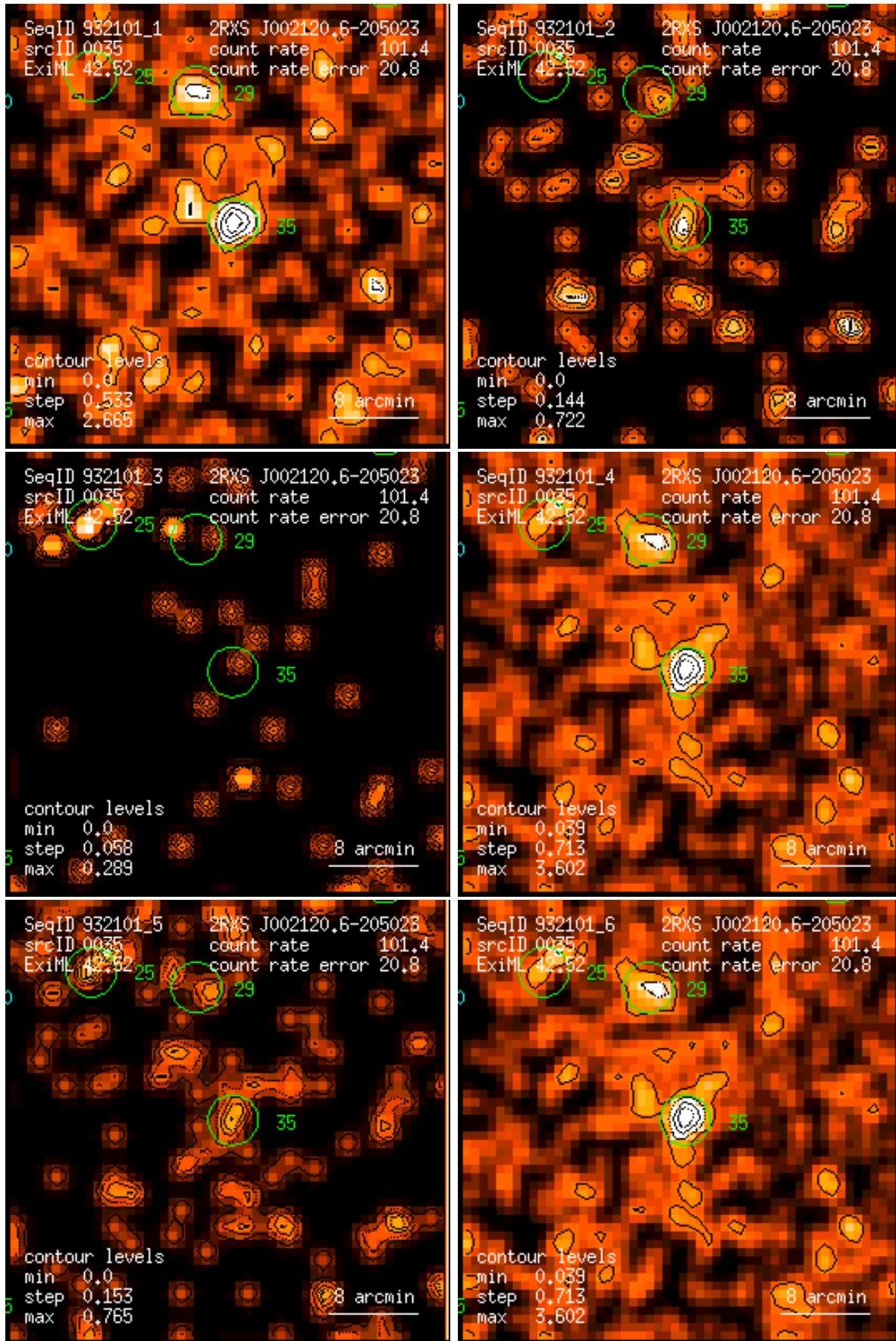
Figure 35: RASS 932101: detection 0035: band rate images, Gaussian filter: (1) PSPC channels 11 – 41, (2) 52 – 90, (3) 91 – 201, (4) 11 – 235, (5) 52 – 201, (6) 11 – 201. Broad band rates in counts/ks. Band rate contour levels in counts/ks/arcmin 2 .
