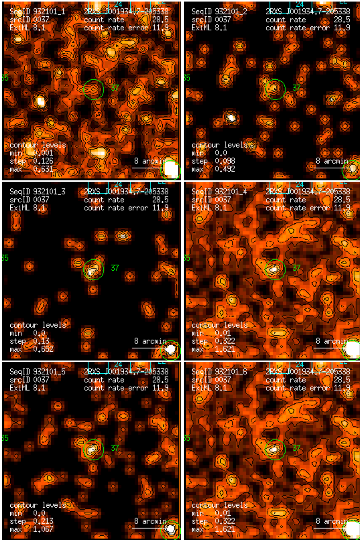
Figure 37: RASS 932101: detection 0037: band rate images, Gaussian filter: (1) PSPC channels 11 – 41, (2) 52 – 90, (3) 91 – 201, (4) 11 – 235, (5) 52 – 201, (6) 11 – 201. Broad band rates in counts/ks. Band rate contour levels in counts/ks/arcmin 2 .
