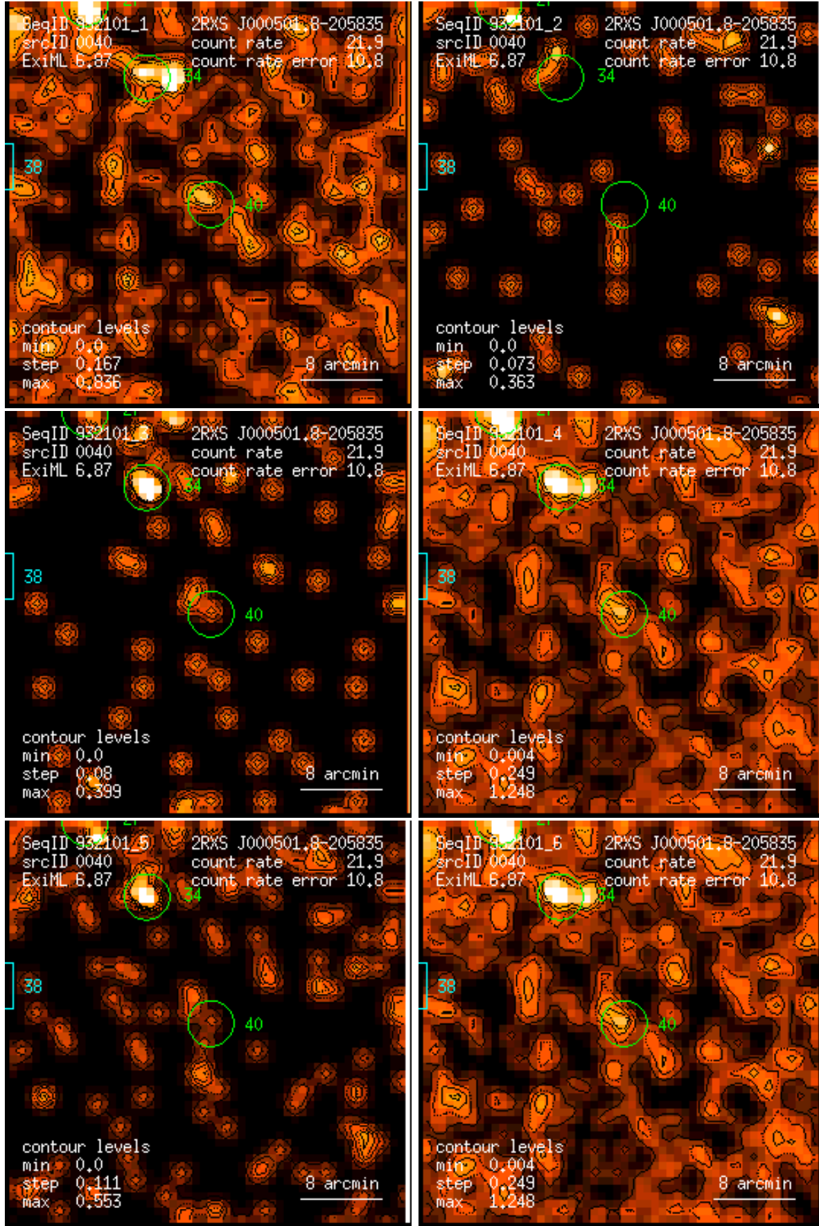
Figure 40: RASS 932101: detection 0040: band rate images, Gaussian filter: (1) PSPC channels 11 – 41, (2) 52 – 90, (3) 91 – 201, (4) 11 – 235, (5) 52 – 201, (6) 11 – 201. Broad band rates in counts/ks. Band rate contour levels in counts/ks/arcmin 2 .
