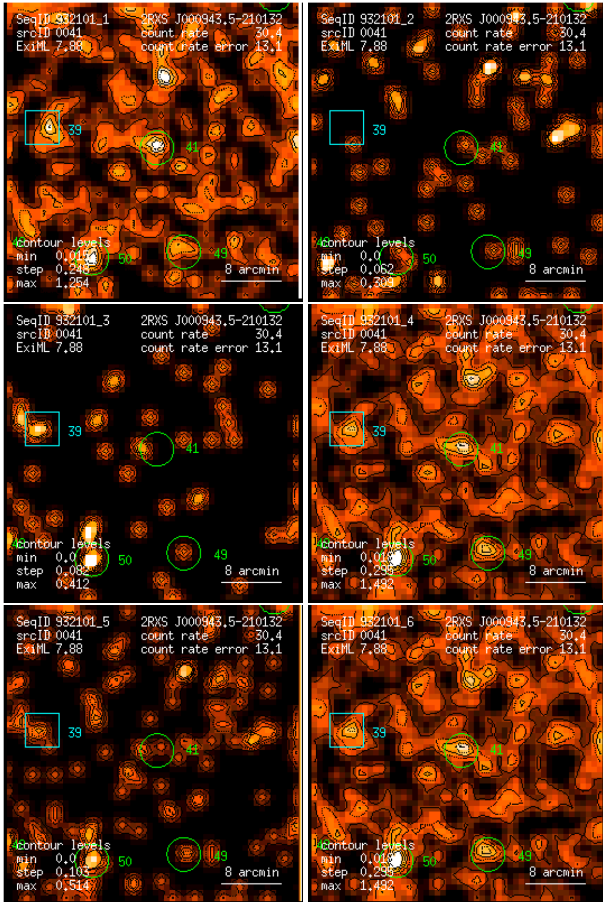
Figure 41: RASS 932101: detection 0041: band rate images, Gaussian filter: (1) PSPC channels 11 – 41, (2) 52 – 90, (3) 91 – 201, (4) 11 – 235, (5) 52 – 201, (6) 11 – 201. Broad band rates in counts/ks. Band rate contour levels in counts/ks/arcmin 2 .
