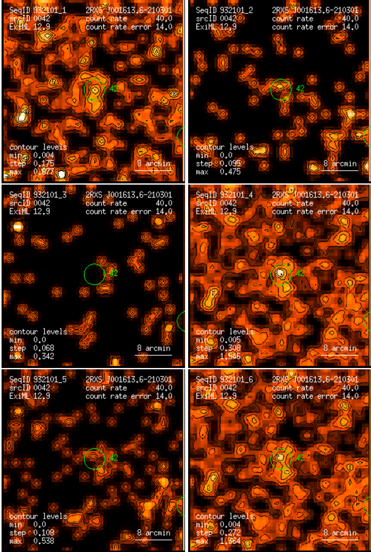
Figure 42: RASS 932101: detection 0042: band rate images, Gaussian filter: (1) PSPC channels 11 – 41, (2) 52 – 90, (3) 91 – 201, (4) 11 – 235, (5) 52 – 201, (6) 11 – 201. Broad band rates in counts/ks. Band rate contour levels in counts/ks/arcmin 2 .
