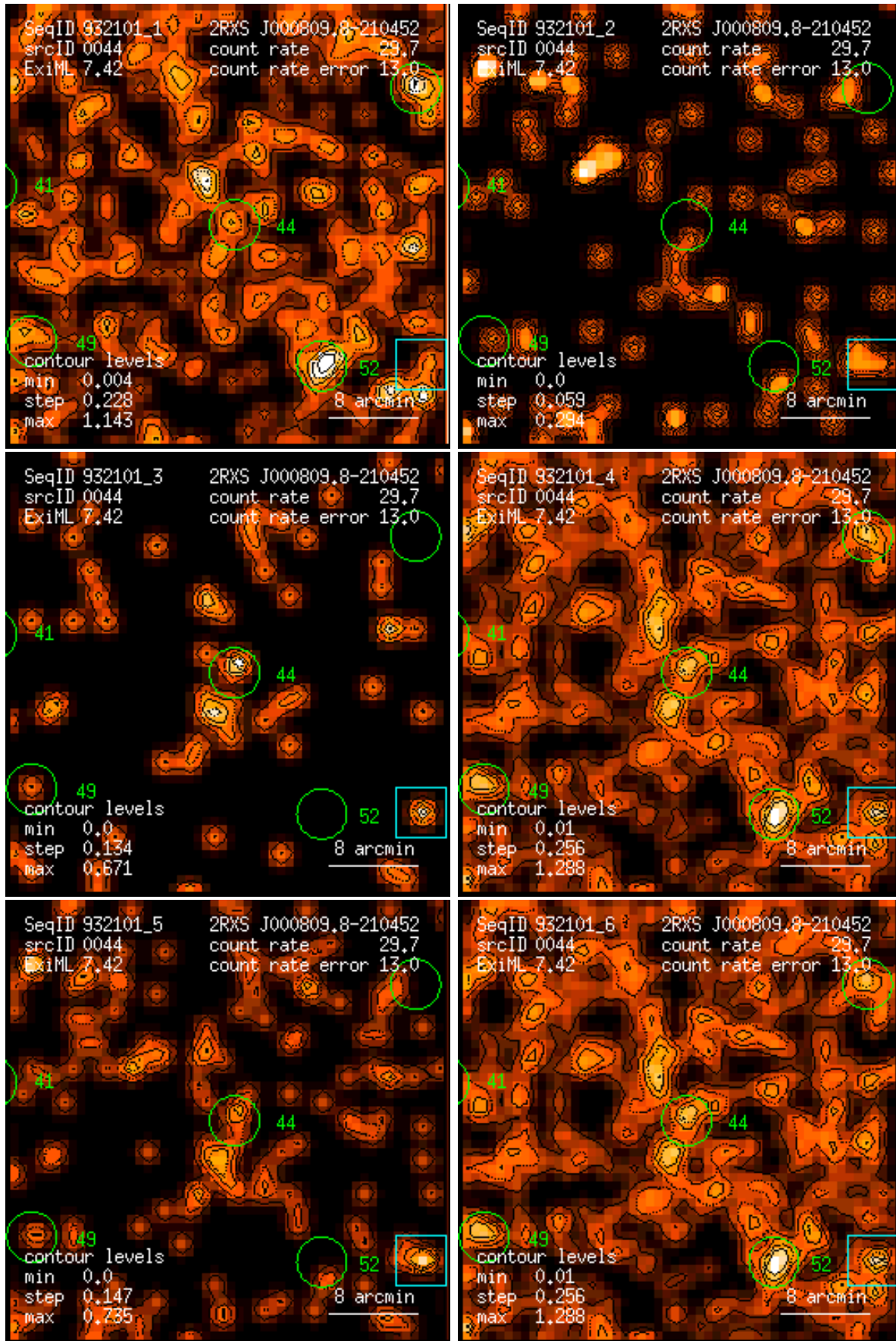
Figure 44: RASS 932101: detection 0044: band rate images, Gaussian filter: (1) PSPC channels 11 – 41, (2) 52 – 90, (3) 91 – 201, (4) 11 – 235, (5) 52 – 201, (6) 11 – 201. Broad band rates in counts/ks. Band rate contour levels in counts/ks/arcmin 2 .
