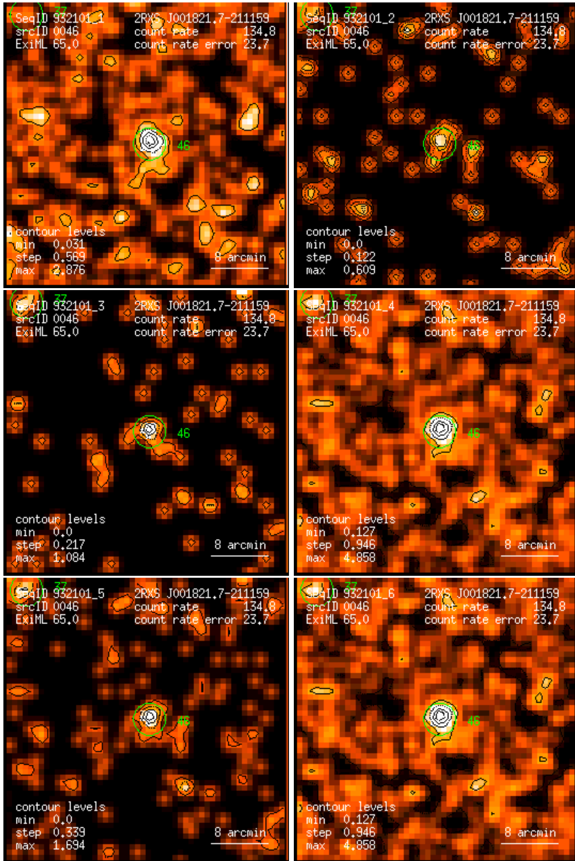
Figure 46: RASS 932101: detection 0046: band rate images, Gaussian filter: (1) PSPC channels 11 – 41, (2) 52 – 90, (3) 91 – 201, (4) 11 – 235, (5) 52 – 201, (6) 11 – 201. Broad band rates in counts/ks. Band rate contour levels in counts/ks/arcmin 2 .
