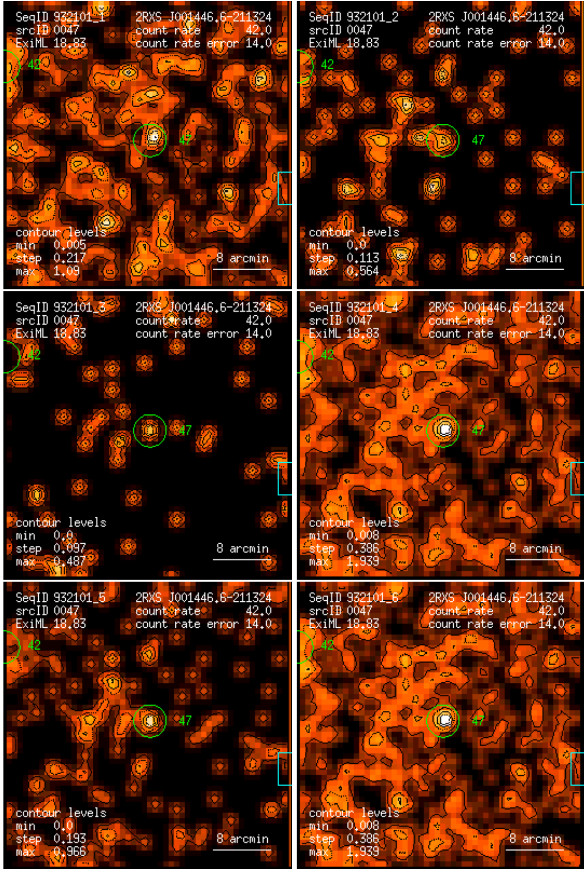
Figure 47: RASS 932101: detection 0047: band rate images, Gaussian filter: (1) PSPC channels 11 – 41, (2) 52 – 90, (3) 91 – 201, (4) 11 – 235, (5) 52 – 201, (6) 11 – 201. Broad band rates in counts/ks. Band rate contour levels in counts/ks/arcmin 2 .
