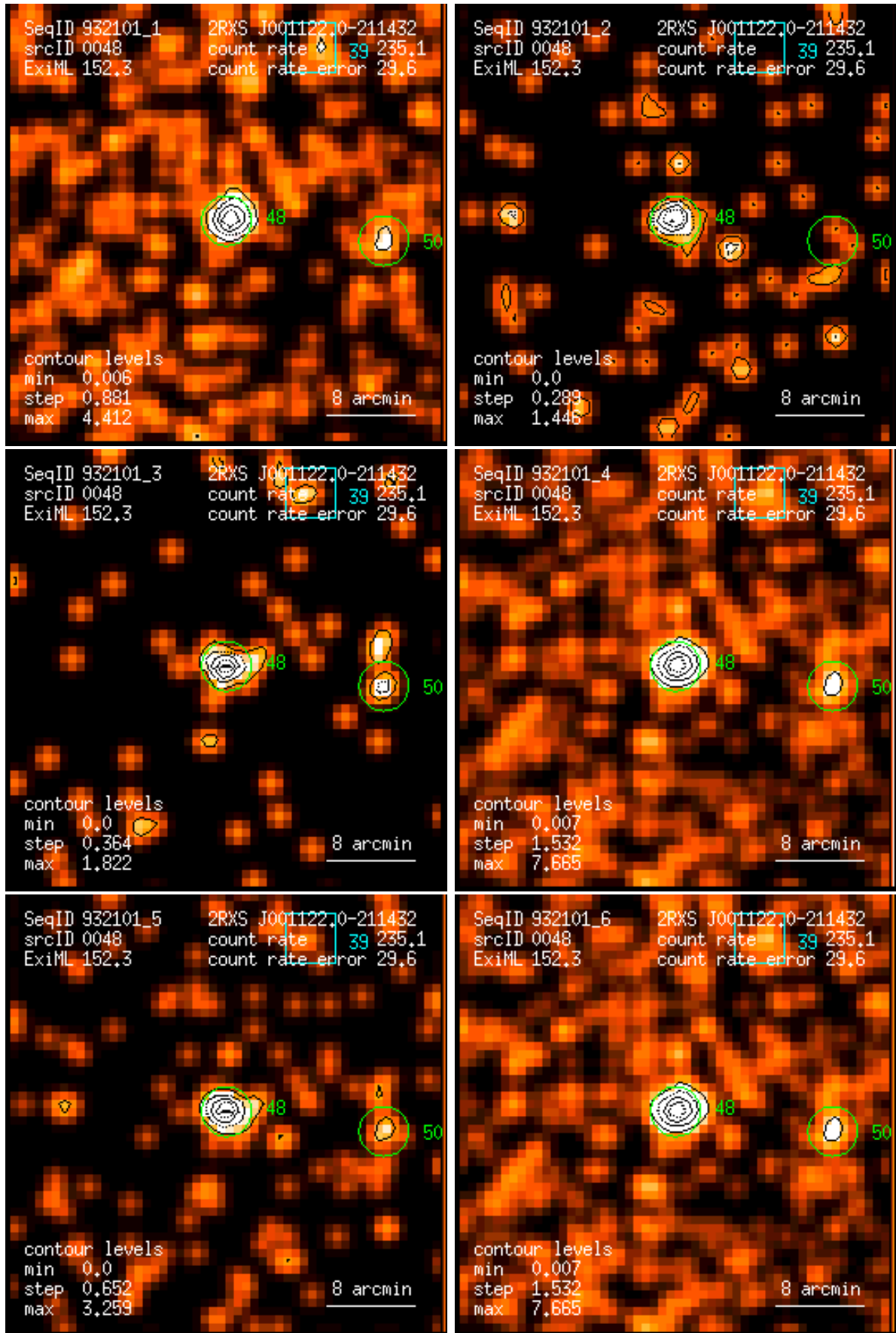
Figure 48: RASS 932101: detection 0048: band rate images, Gaussian filter: (1) PSPC channels 11 – 41, (2) 52 – 90, (3) 91 – 201, (4) 11 – 235, (5) 52 – 201, (6) 11 – 201. Broad band rates in counts/ks. Band rate contour levels in counts/ks/arcmin 2 .
