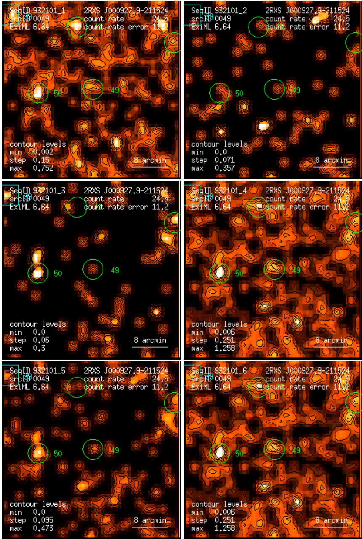
Figure 49: RASS 932101: detection 0049: band rate images, Gaussian filter: (1) PSPC channels 11 – 41, (2) 52 – 90, (3) 91 – 201, (4) 11 – 235, (5) 52 – 201, (6) 11 – 201. Broad band rates in counts/ks. Band rate contour levels in counts/ks/arcmin 2 .
