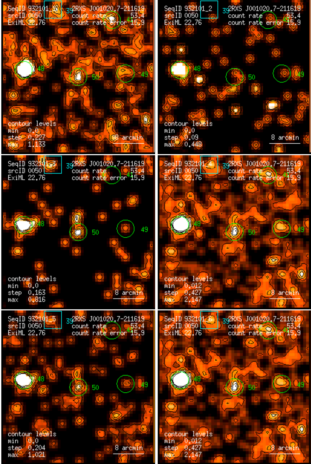
Figure 50: RASS 932101: detection 0050: band rate images, Gaussian filter: (1) PSPC channels 11 – 41, (2) 52 – 90, (3) 91 – 201, (4) 11 – 235, (5) 52 – 201, (6) 11 – 201. Broad band rates in counts/ks. Band rate contour levels in counts/ks/arcmin 2 .
