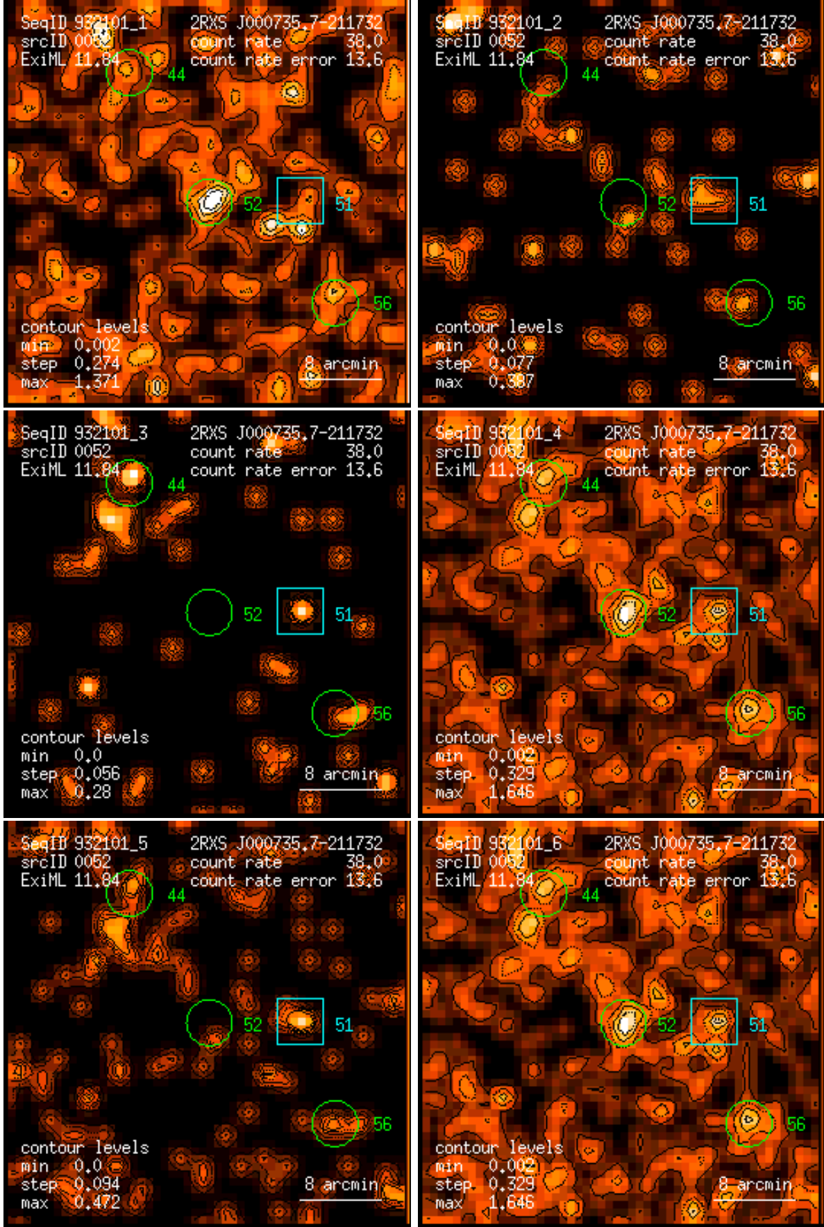
Figure 52: RASS 932101: detection 0052: band rate images, Gaussian filter: (1) PSPC channels 11 – 41, (2) 52 – 90, (3) 91 – 201, (4) 11 – 235, (5) 52 – 201, (6) 11 – 201. Broad band rates in counts/ks. Band rate contour levels in counts/ks/arcmin 2 .
