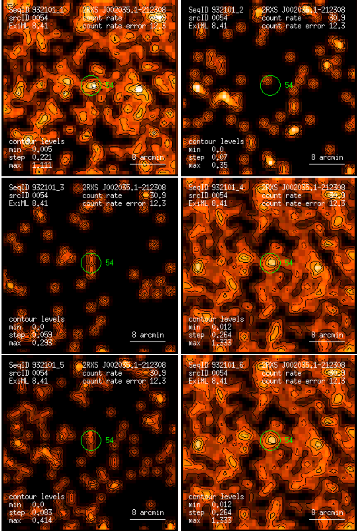
Figure 54: RASS 932101: detection 0054: band rate images, Gaussian filter: (1) PSPC channels 11 – 41, (2) 52 – 90, (3) 91 – 201, (4) 11 – 235, (5) 52 – 201, (6) 11 – 201. Broad band rates in counts/ks. Band rate contour levels in counts/ks/arcmin 2 .
