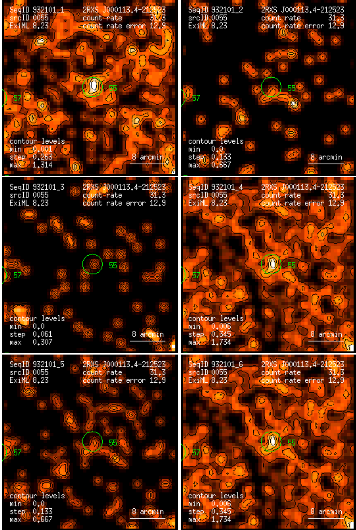
Figure 55: RASS 932101: detection 0055: band rate images, Gaussian filter: (1) PSPC channels 11 – 41, (2) 52 – 90, (3) 91 – 201, (4) 11 – 235, (5) 52 – 201, (6) 11 – 201. Broad band rates in counts/ks. Band rate contour levels in counts/ks/arcmin 2 .
