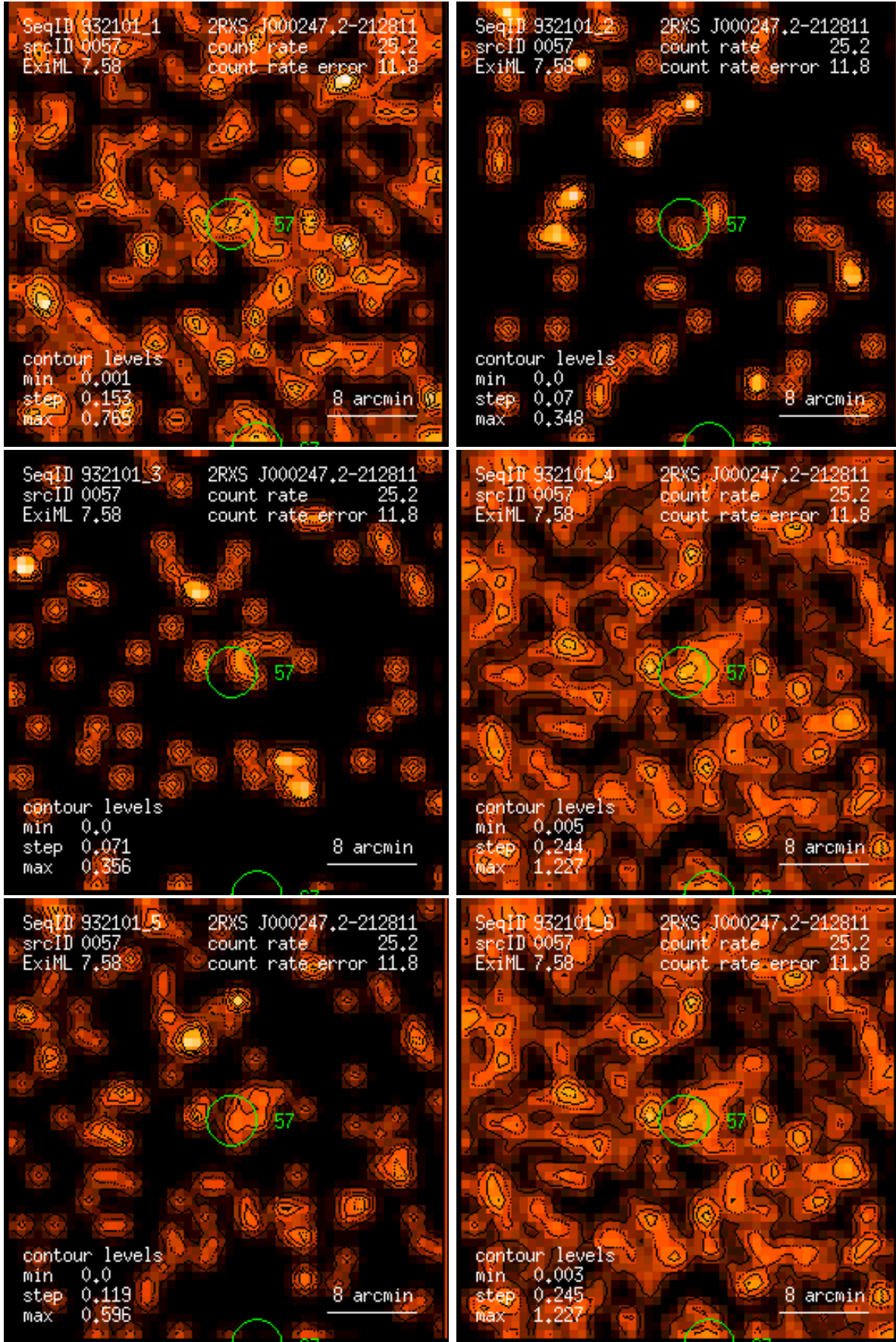
Figure 57: RASS 932101: detection 0057: band rate images, Gaussian filter: (1) PSPC channels 11 – 41, (2) 52 – 90, (3) 91 – 201, (4) 11 – 235, (5) 52 – 201, (6) 11 – 201. Broad band rates in counts/ks. Band rate contour levels in counts/ks/arcmin 2 .
