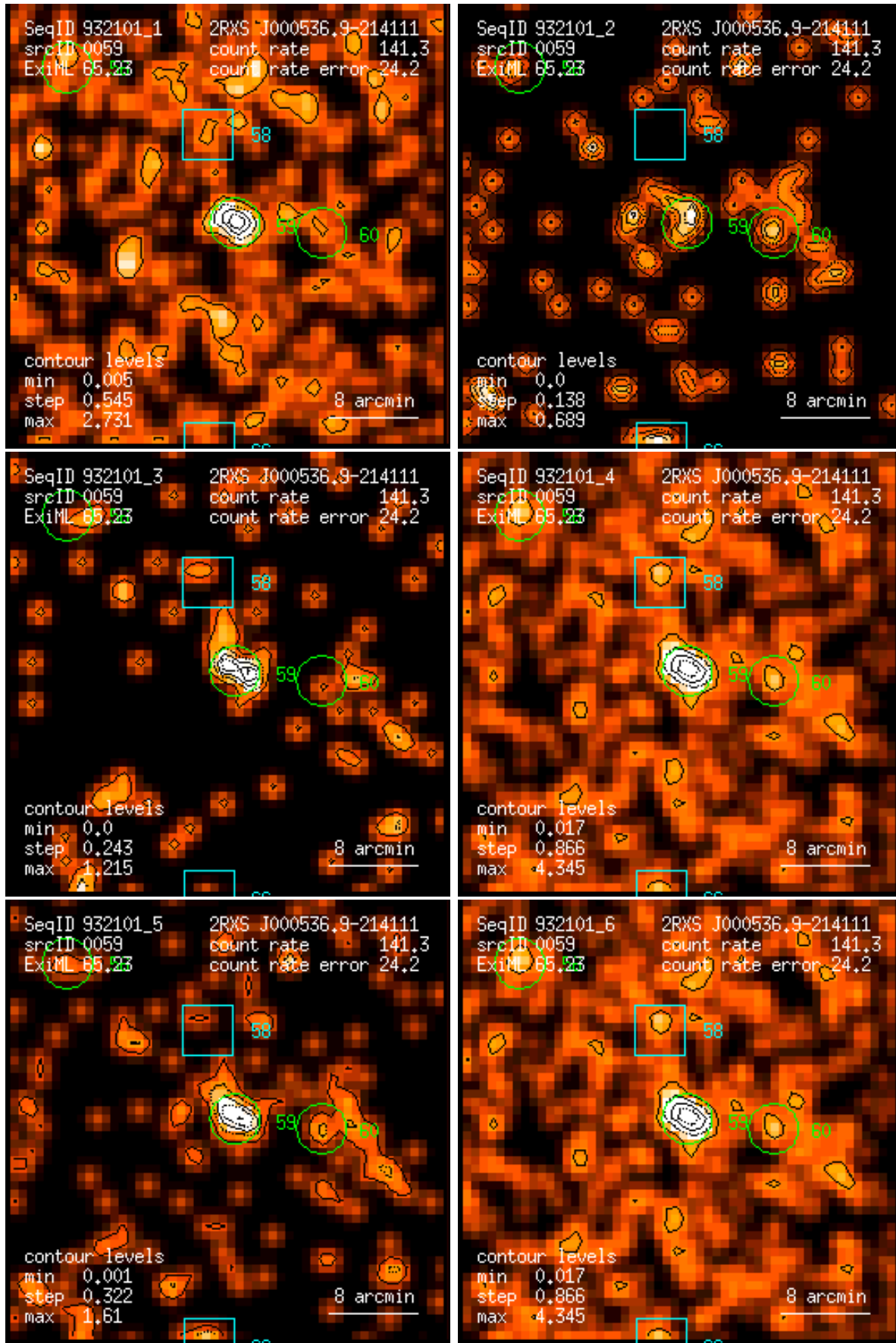
Figure 59: RASS 932101: detection 0059: band rate images, Gaussian filter: (1) PSPC channels 11 – 41, (2) 52 – 90, (3) 91 – 201, (4) 11 – 235, (5) 52 – 201, (6) 11 – 201. Broad band rates in counts/ks. Band rate contour levels in counts/ks/arcmin 2 .
