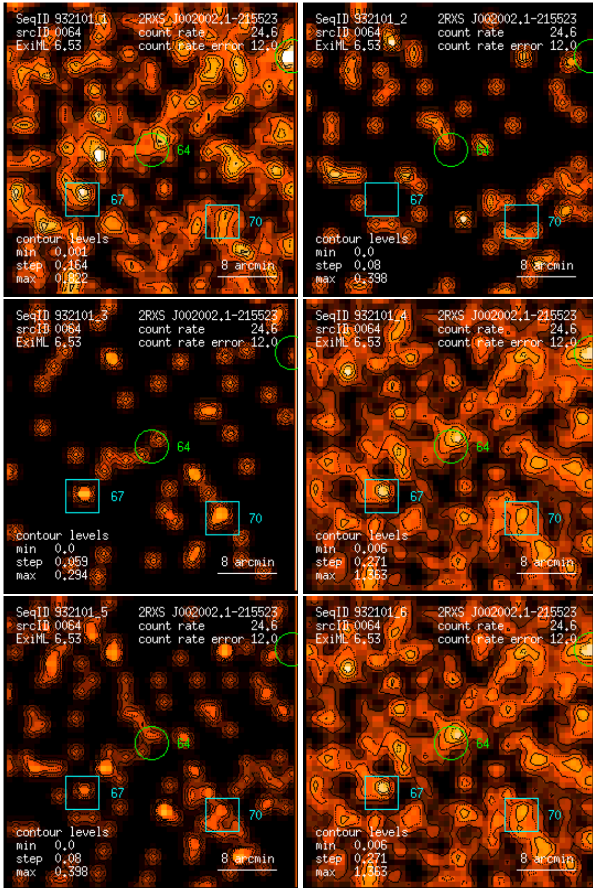
Figure 64: RASS 932101: detection 0064: band rate images, Gaussian filter: (1) PSPC channels 11 – 41, (2) 52 – 90, (3) 91 – 201, (4) 11 – 235, (5) 52 – 201, (6) 11 – 201. Broad band rates in counts/ks. Band rate contour levels in counts/ks/arcmin 2 .
