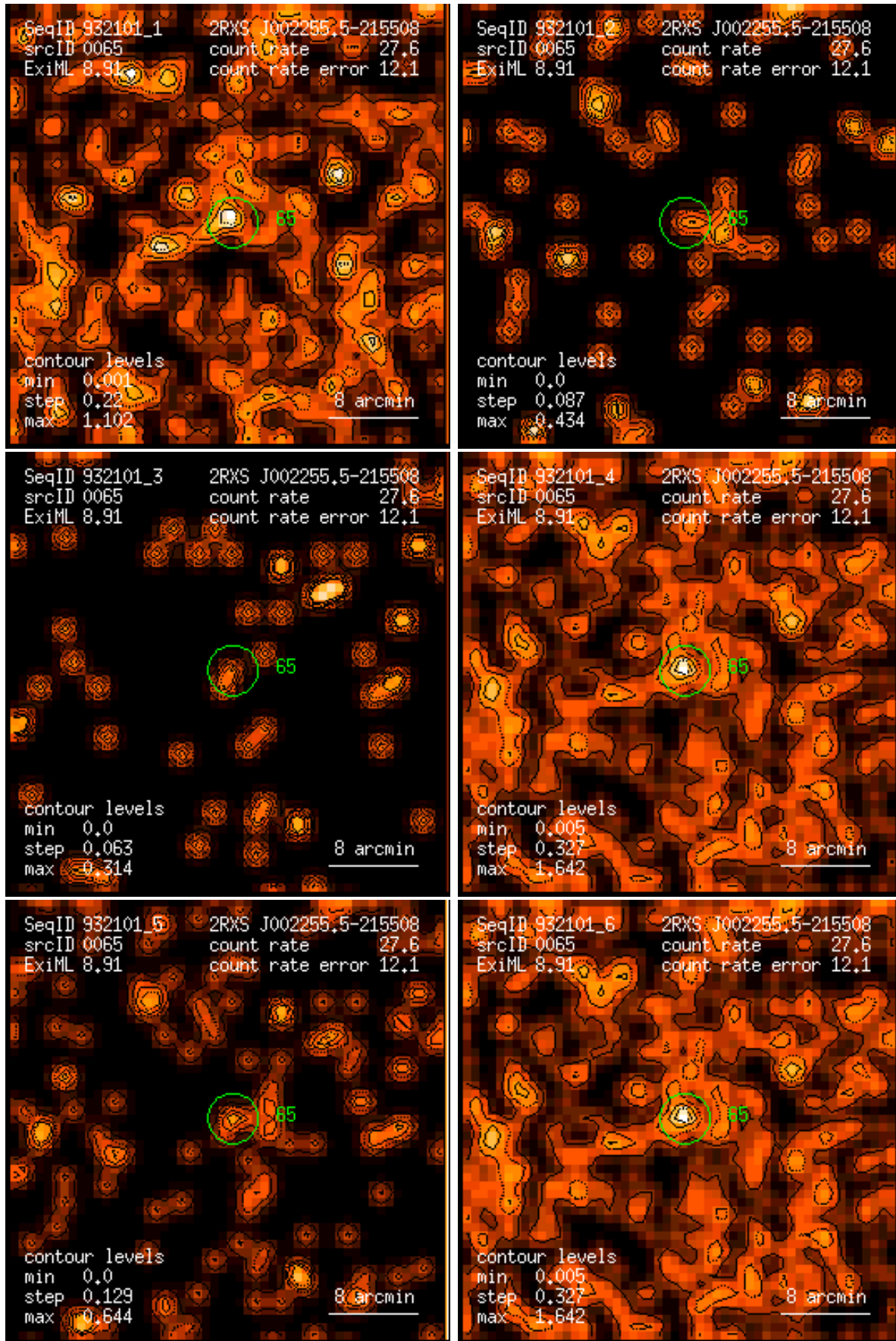
Figure 65: RASS 932101: detection 0065: band rate images, Gaussian filter: (1) PSPC channels 11 – 41, (2) 52 – 90, (3) 91 – 201, (4) 11 – 235, (5) 52 – 201, (6) 11 – 201. Broad band rates in counts/ks. Band rate contour levels in counts/ks/arcmin 2 .
