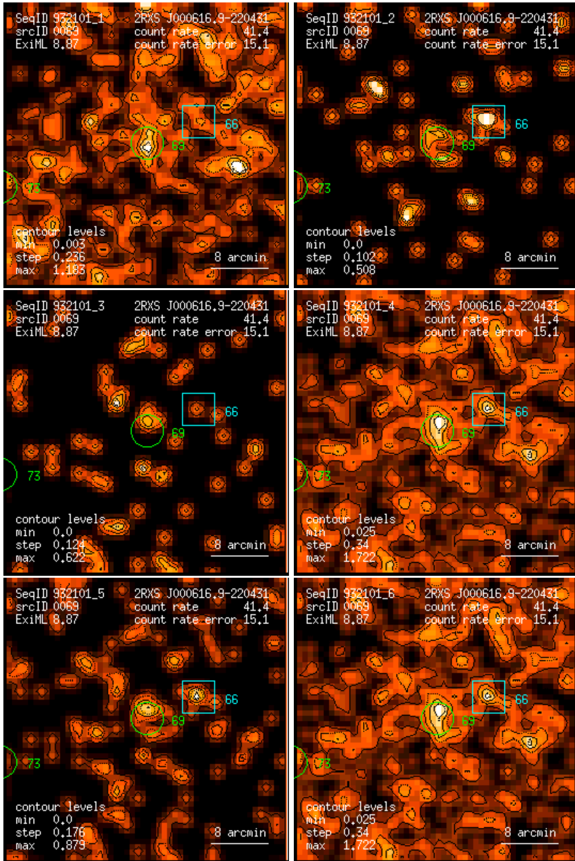
Figure 69: RASS 932101: detection 0069: band rate images, Gaussian filter: (1) PSPC channels 11 – 41, (2) 52 – 90, (3) 91 – 201, (4) 11 – 235, (5) 52 – 201, (6) 11 – 201. Broad band rates in counts/ks. Band rate contour levels in counts/ks/arcmin 2 .
