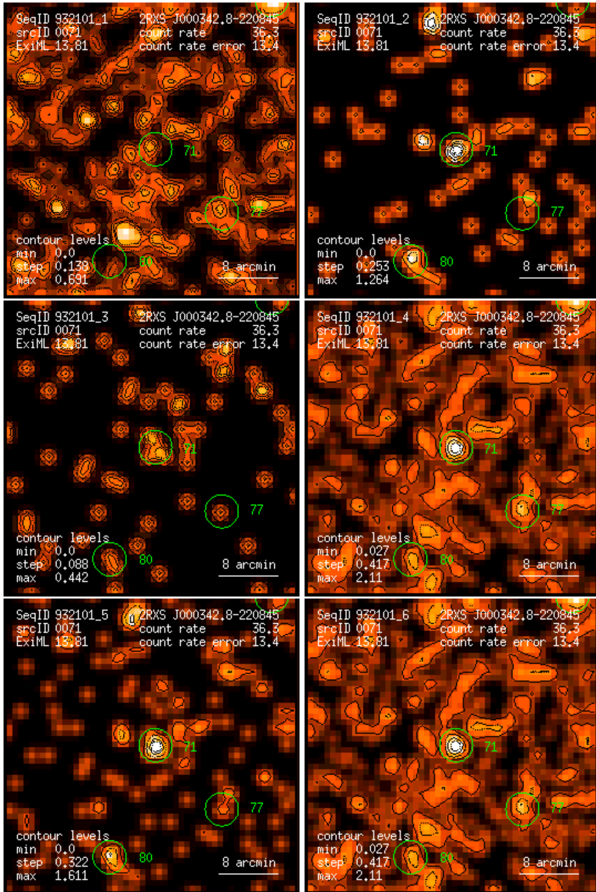
Figure 71: RASS 932101: detection 0071: band rate images, Gaussian filter: (1) PSPC channels 11 – 41, (2) 52 – 90, (3) 91 – 201, (4) 11 – 235, (5) 52 – 201, (6) 11 – 201. Broad band rates in counts/ks. Band rate contour levels in counts/ks/arcmin 2 .
