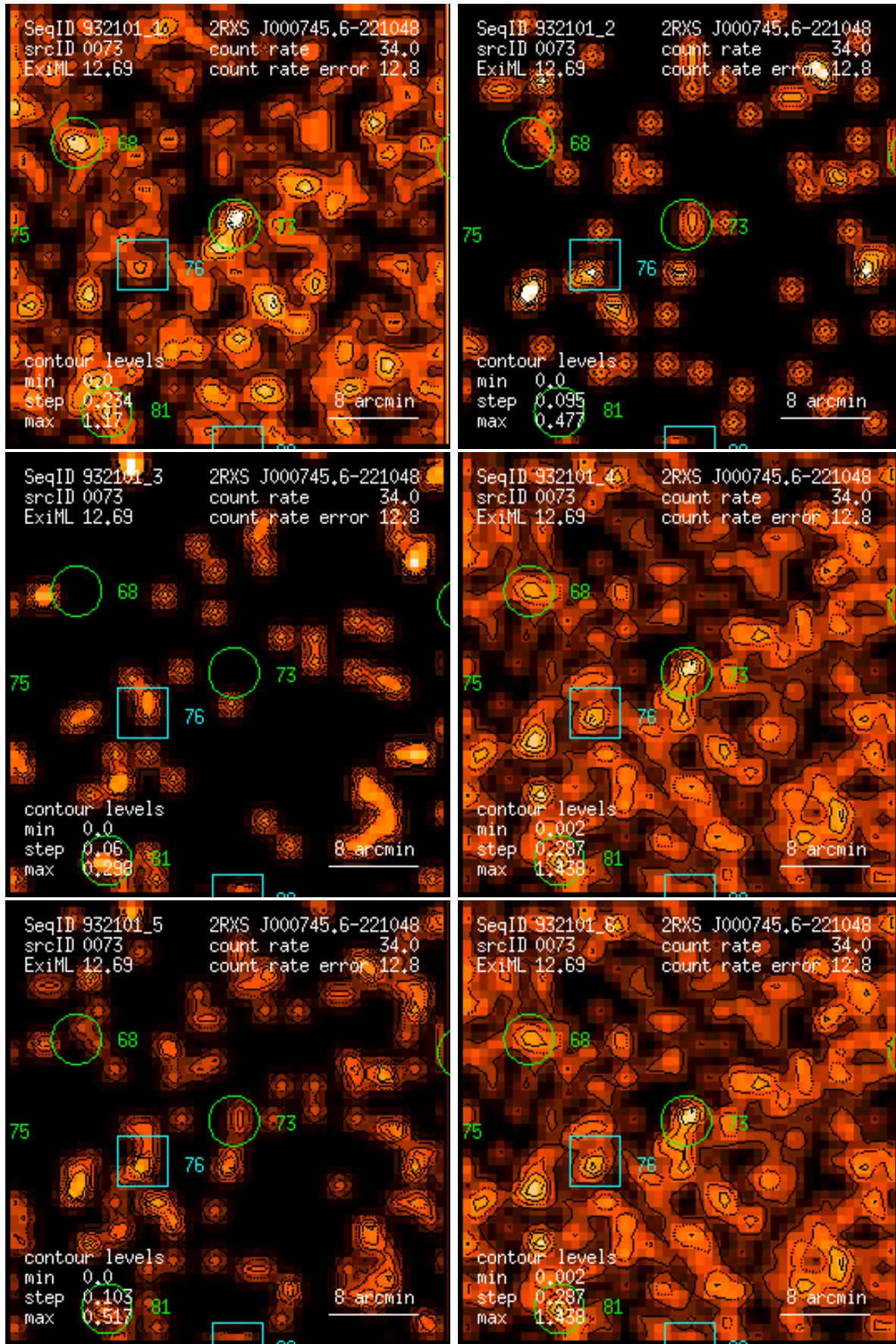
Figure 73: RASS 932101: detection 0073: band rate images, Gaussian filter: (1) PSPC channels 11 – 41, (2) 52 – 90, (3) 91 – 201, (4) 11 – 235, (5) 52 – 201, (6) 11 – 201. Broad band rates in counts/ks. Band rate contour levels in counts/ks/arcmin 2 .
