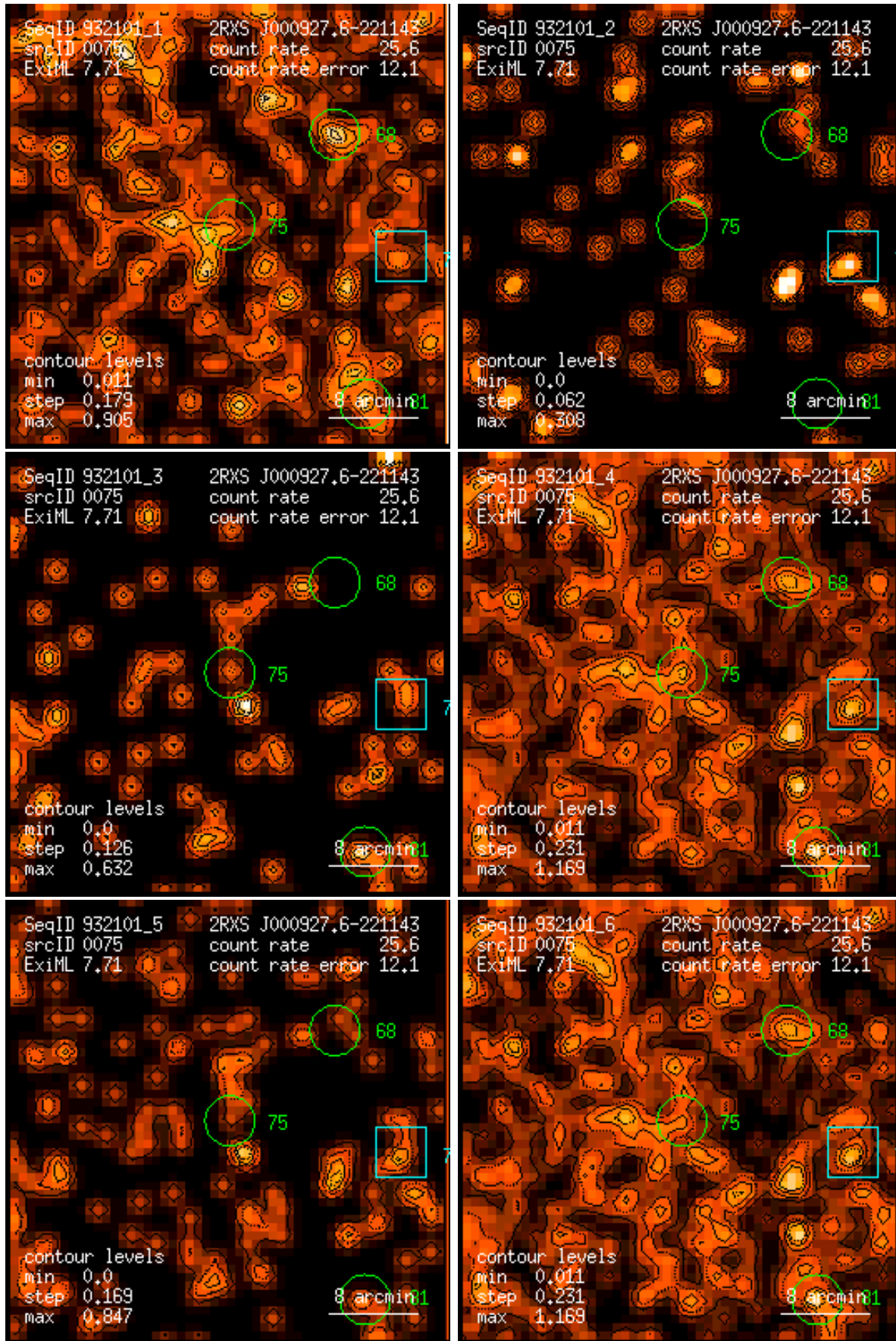
Figure 75: RASS 932101: detection 0075: band rate images, Gaussian filter: (1) PSPC channels 11 – 41, (2) 52 – 90, (3) 91 – 201, (4) 11 – 235, (5) 52 – 201, (6) 11 – 201. Broad band rates in counts/ks. Band rate contour levels in counts/ks/arcmin 2 .
