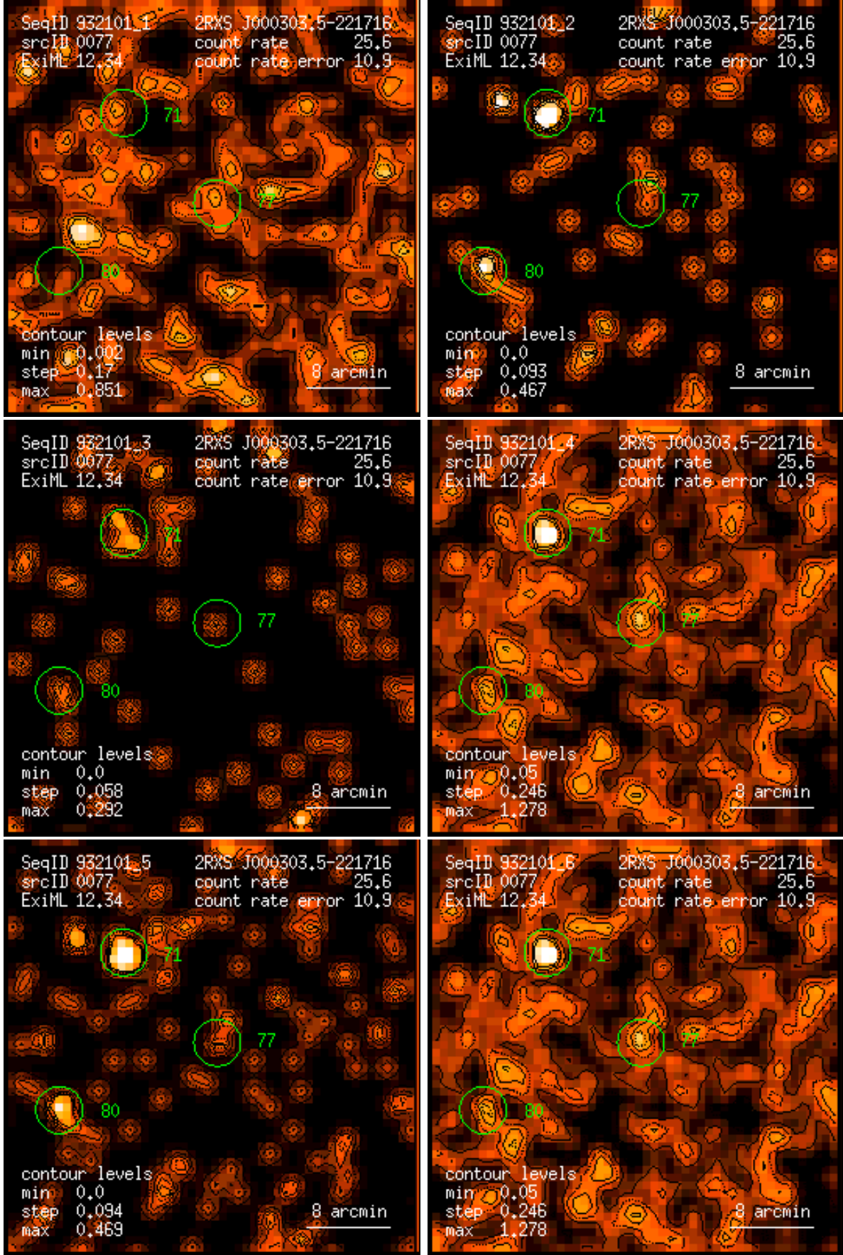
Figure 77: RASS 932101: detection 0077: band rate images, Gaussian filter: (1) PSPC channels 11 – 41, (2) 52 – 90, (3) 91 – 201, (4) 11 – 235, (5) 52 – 201, (6) 11 – 201. Broad band rates in counts/ks. Band rate contour levels in counts/ks/arcmin 2 .
