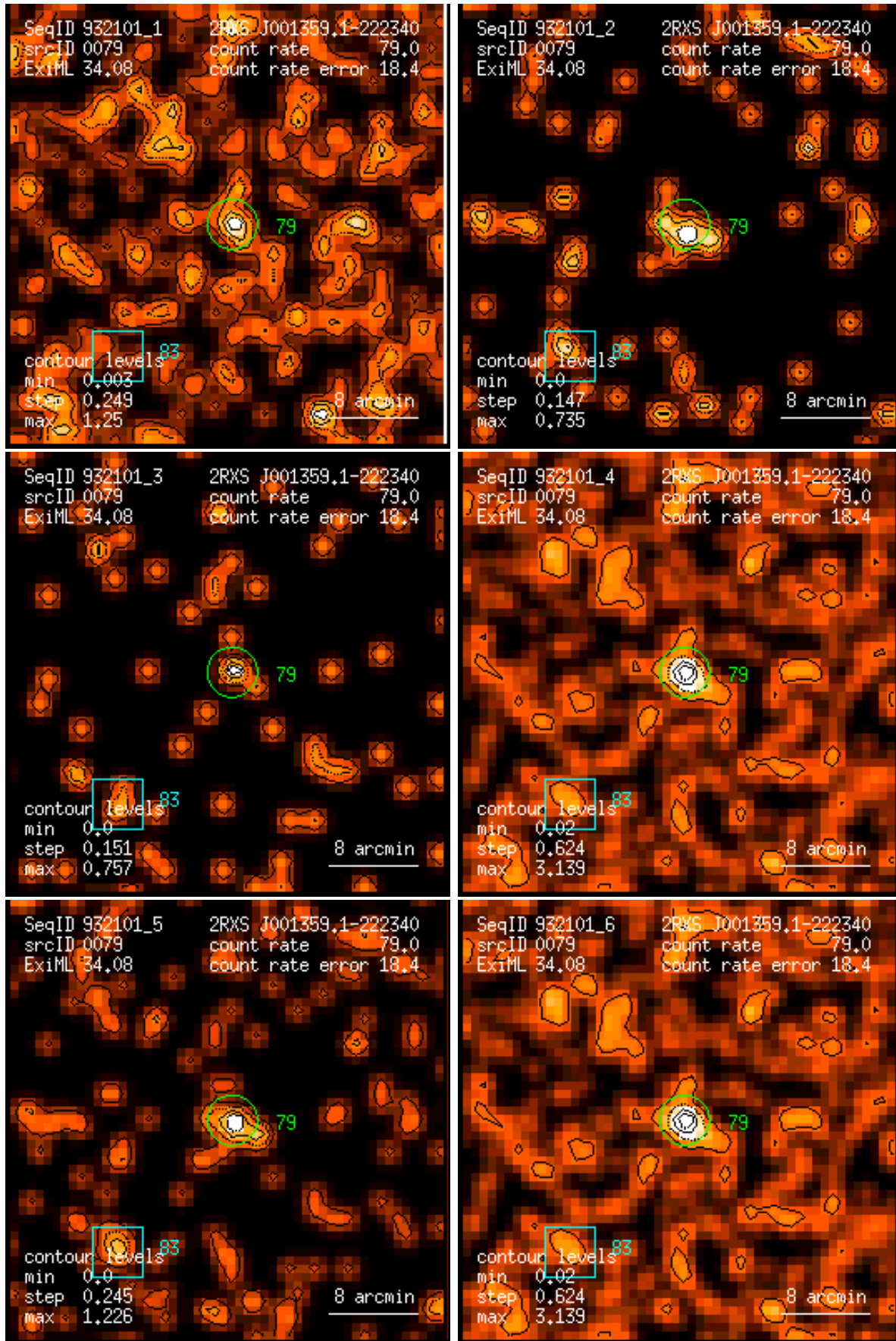
Figure 79: RASS 932101: detection 0079: band rate images, Gaussian filter: (1) PSPC channels 11 – 41, (2) 52 – 90, (3) 91 – 201, (4) 11 – 235, (5) 52 – 201, (6) 11 – 201. Broad band rates in counts/ks. Band rate contour levels in counts/ks/arcmin 2 .
