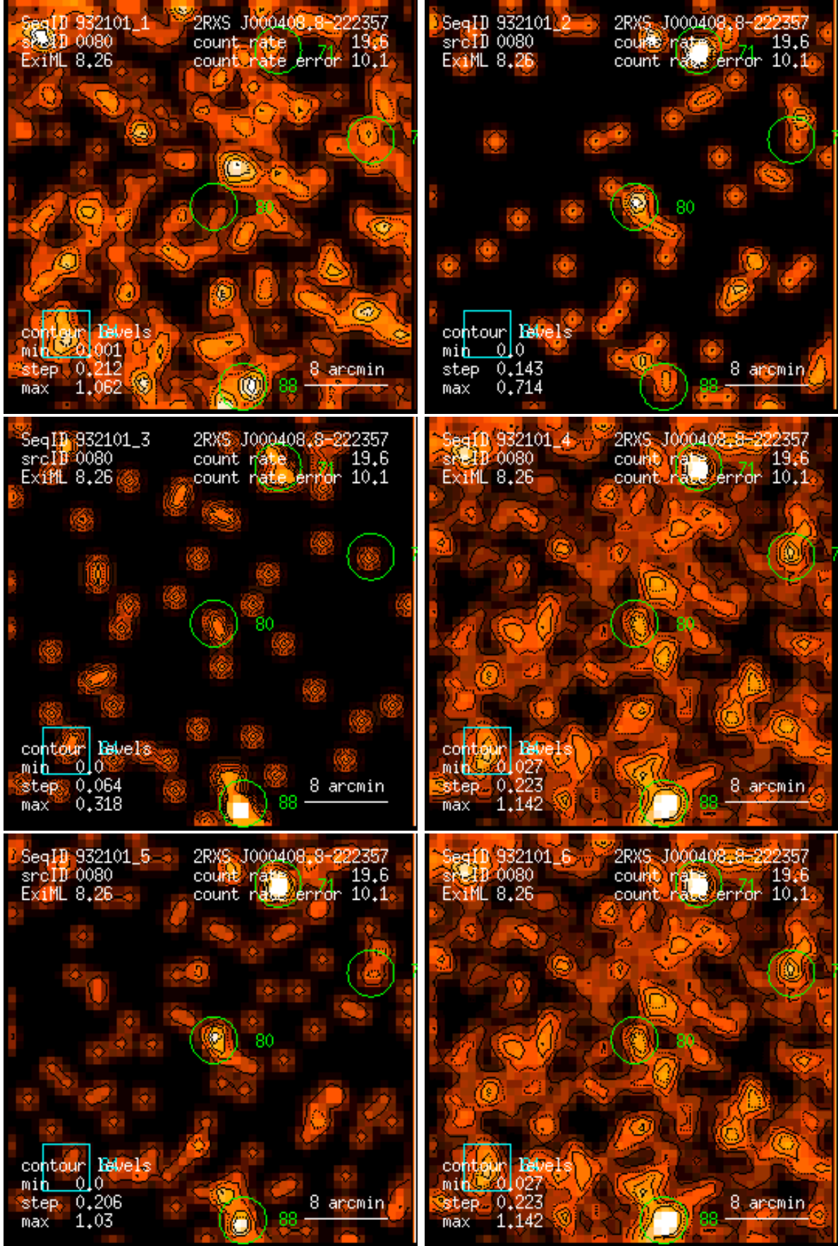
Figure 80: RASS 932101: detection 0080: band rate images, Gaussian filter: (1) PSPC channels 11 – 41, (2) 52 – 90, (3) 91 – 201, (4) 11 – 235, (5) 52 – 201, (6) 11 – 201. Broad band rates in counts/ks. Band rate contour levels in counts/ks/arcmin 2 .
