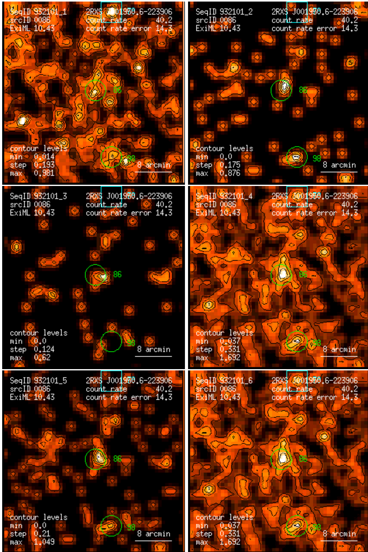
Figure 86: RASS 932101: detection 0086: band rate images, Gaussian filter: (1) PSPC channels 11 – 41, (2) 52 – 90, (3) 91 – 201, (4) 11 – 235, (5) 52 – 201, (6) 11 – 201. Broad band rates in counts/ks. Band rate contour levels in counts/ks/arcmin 2 .
