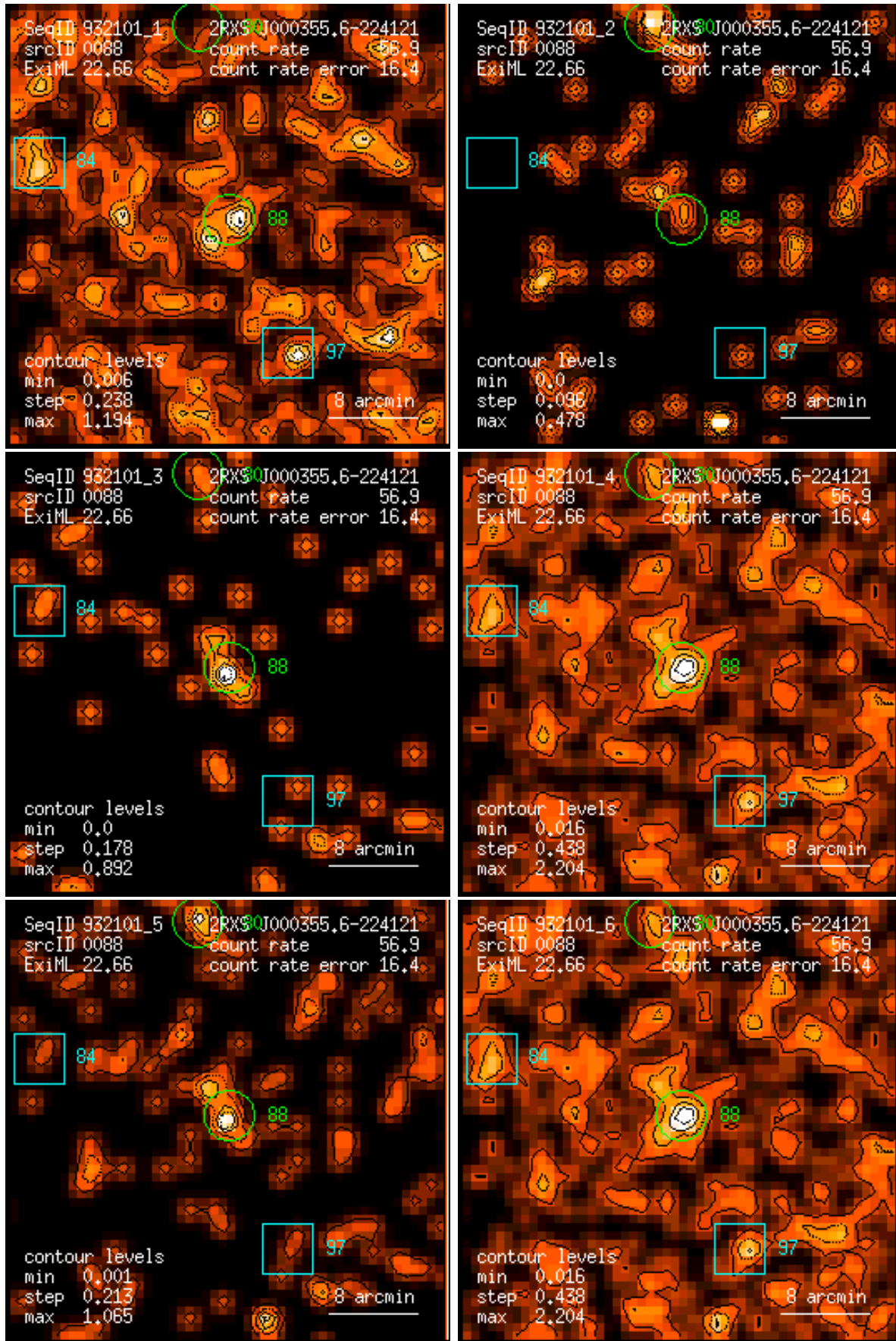
Figure 88: RASS 932101: detection 0088: band rate images, Gaussian filter: (1) PSPC channels 11 – 41, (2) 52 – 90, (3) 91 – 201, (4) 11 – 235, (5) 52 – 201, (6) 11 – 201. Broad band rates in counts/ks. Band rate contour levels in counts/ks/arcmin 2 .
