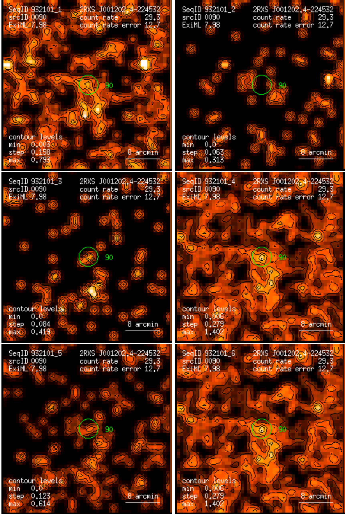
Figure 90: RASS 932101: detection 0090: band rate images, Gaussian filter: (1) PSPC channels 11 – 41, (2) 52 – 90, (3) 91 – 201, (4) 11 – 235, (5) 52 – 201, (6) 11 – 201. Broad band rates in counts/ks. Band rate contour levels in counts/ks/arcmin 2 .
