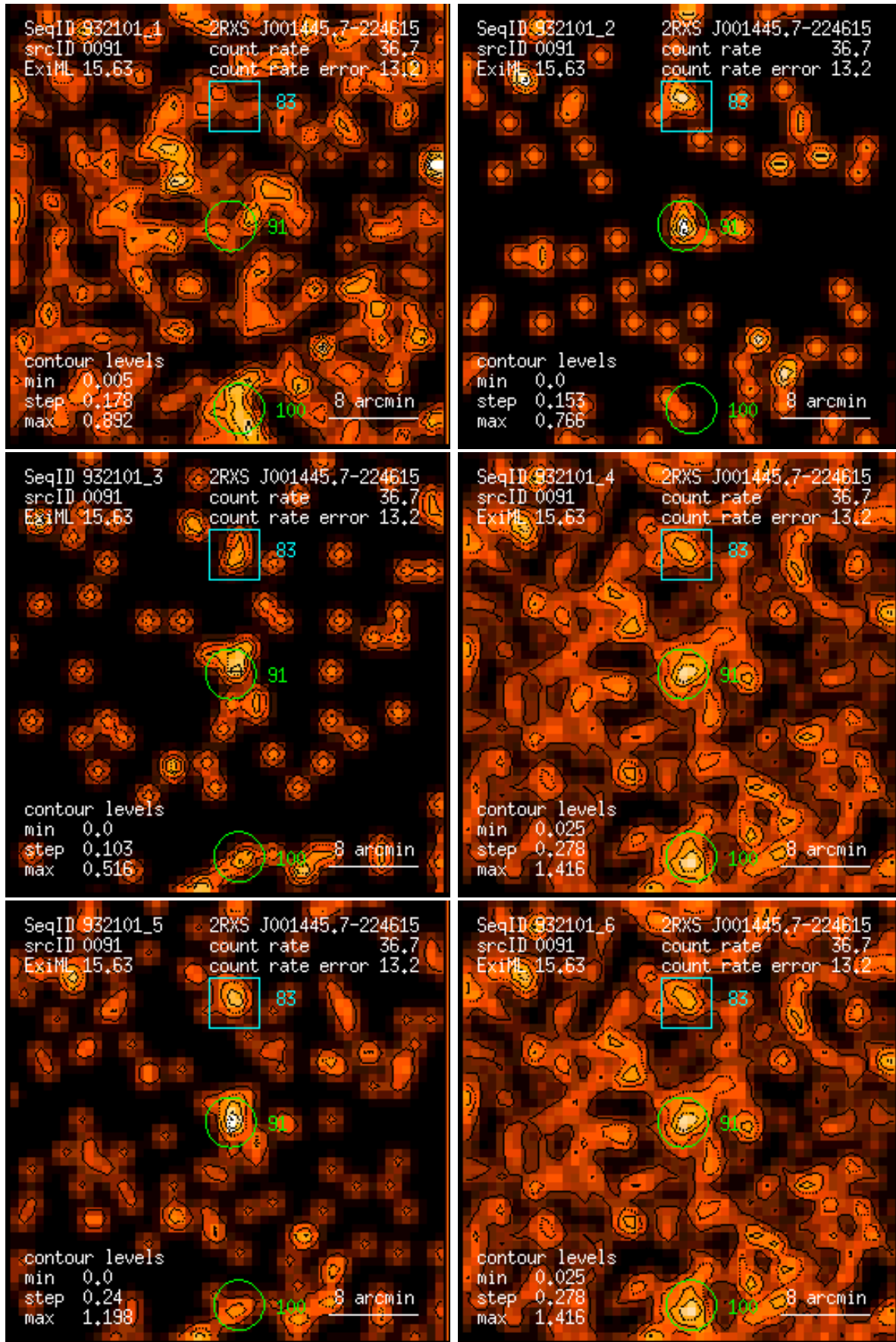
Figure 91: RASS 932101: detection 0091: band rate images, Gaussian filter: (1) PSPC channels 11 – 41, (2) 52 – 90, (3) 91 – 201, (4) 11 – 235, (5) 52 – 201, (6) 11 – 201. Broad band rates in counts/ks. Band rate contour levels in counts/ks/arcmin 2 .
