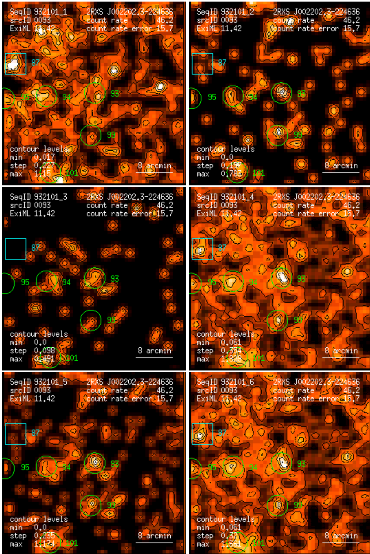
Figure 93: RASS 932101: detection 0093: band rate images, Gaussian filter: (1) PSPC channels 11 – 41, (2) 52 – 90, (3) 91 – 201, (4) 11 – 235, (5) 52 – 201, (6) 11 – 201. Broad band rates in counts/ks. Band rate contour levels in counts/ks/arcmin 2 .
