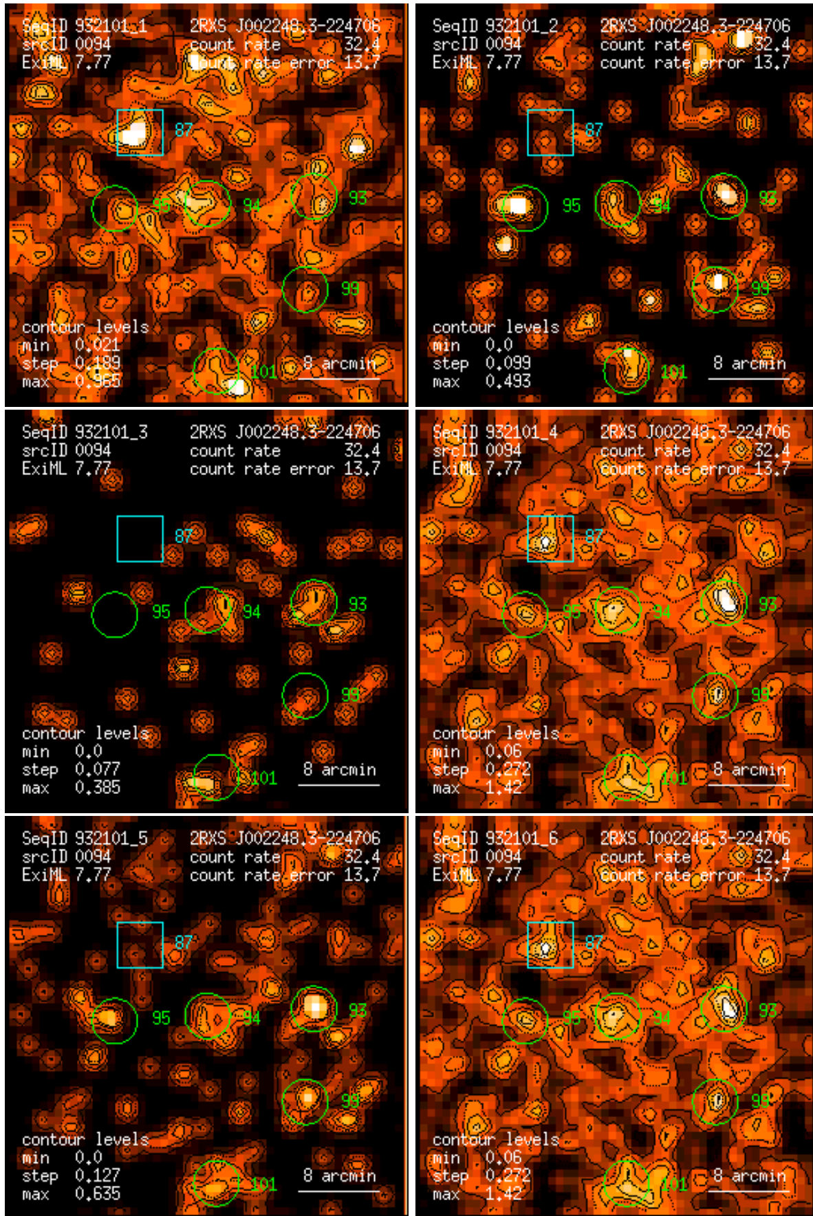
Figure 94: RASS 932101: detection 0094: band rate images, Gaussian filter: (1) PSPC channels 11 – 41, (2) 52 – 90, (3) 91 – 201, (4) 11 – 235, (5) 52 – 201, (6) 11 – 201. Broad band rates in counts/ks. Band rate contour levels in counts/ks/arcmin 2 .
