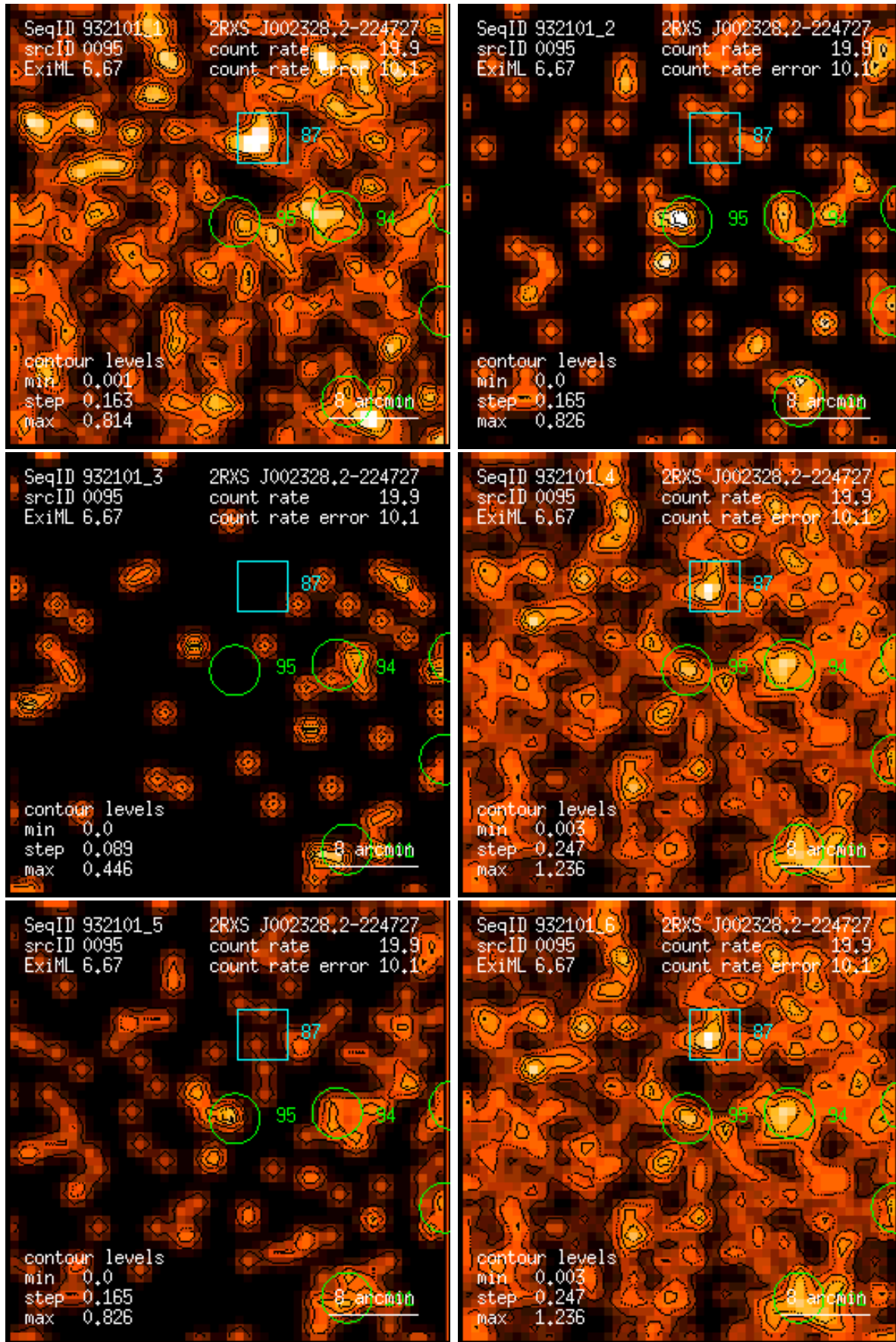
Figure 95: RASS 932101: detection 0095: band rate images, Gaussian filter: (1) PSPC channels 11 – 41, (2) 52 – 90, (3) 91 – 201, (4) 11 – 235, (5) 52 – 201, (6) 11 – 201. Broad band rates in counts/ks. Band rate contour levels in counts/ks/arcmin 2 .
