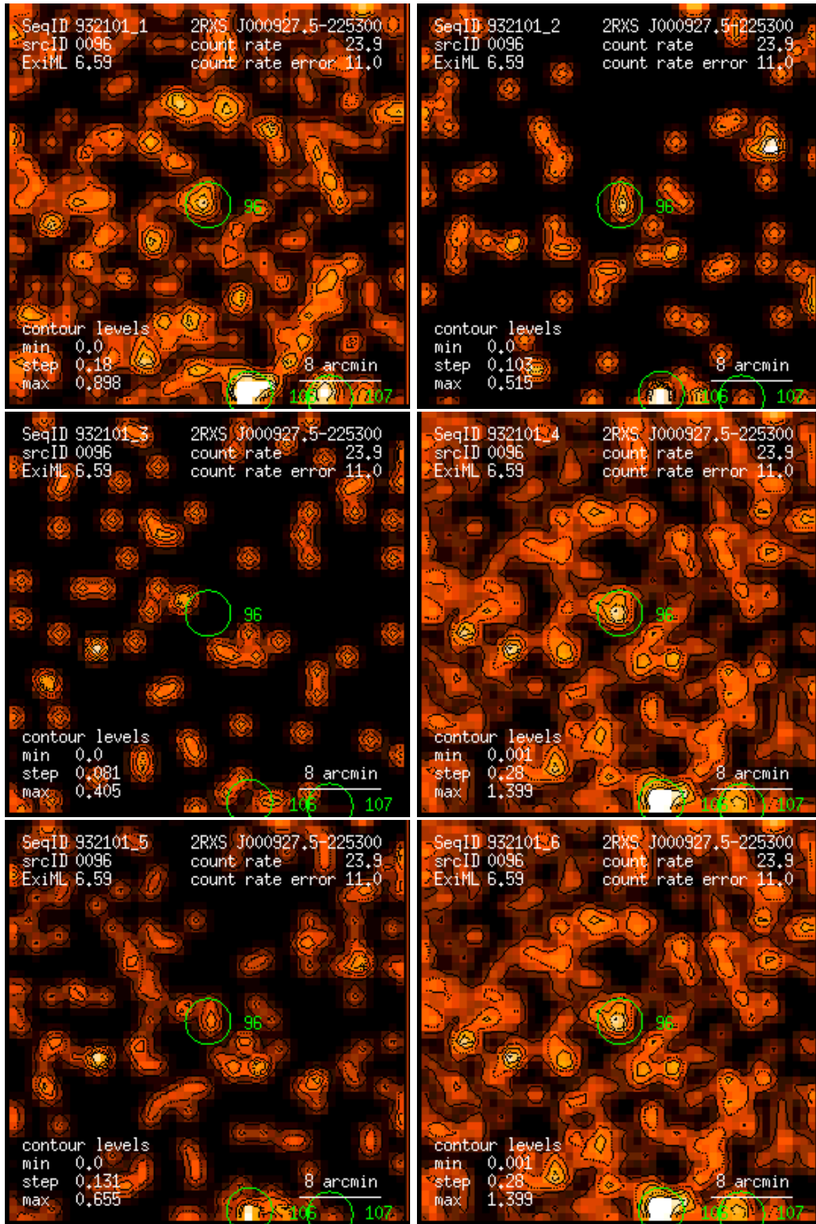
Figure 96: RASS 932101: detection 0096: band rate images, Gaussian filter: (1) PSPC channels 11 – 41, (2) 52 – 90, (3) 91 – 201, (4) 11 – 235, (5) 52 – 201, (6) 11 – 201. Broad band rates in counts/ks. Band rate contour levels in counts/ks/arcmin 2 .
