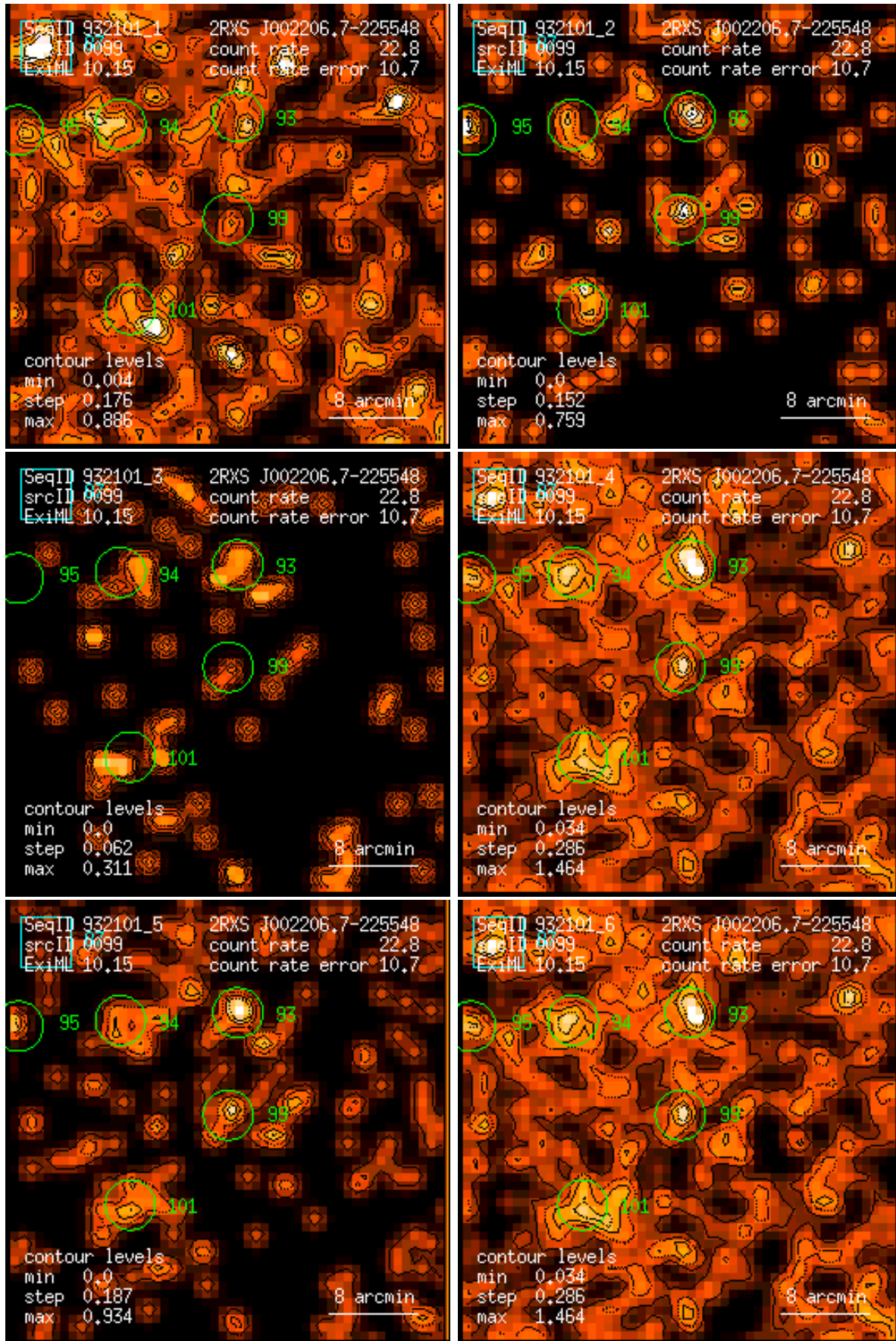
Figure 99: RASS 932101: detection 0099: band rate images, Gaussian filter: (1) PSPC channels 11 – 41, (2) 52 – 90, (3) 91 – 201, (4) 11 – 235, (5) 52 – 201, (6) 11 – 201. Broad band rates in counts/ks. Band rate contour levels in counts/ks/arcmin 2 .
