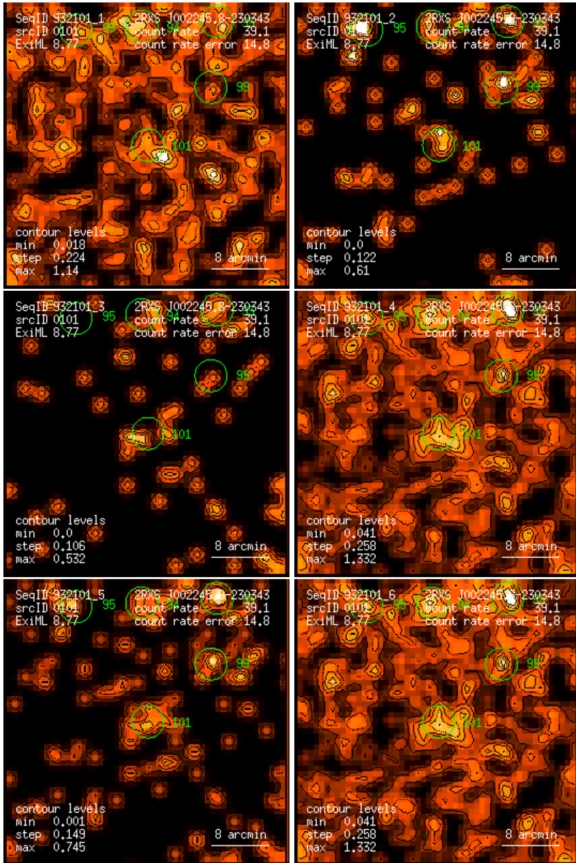
Figure 101: RASS 932101: detection 0101: band rate images, Gaussian filter: (1) PSPC channels 11 – 41, (2) 52 – 90, (3) 91 – 201, (4) 11 – 235, (5) 52 – 201, (6) 11 – 201. Broad band rates in counts/ks. Band rate contour levels in counts/ks/arcmin 2 .
