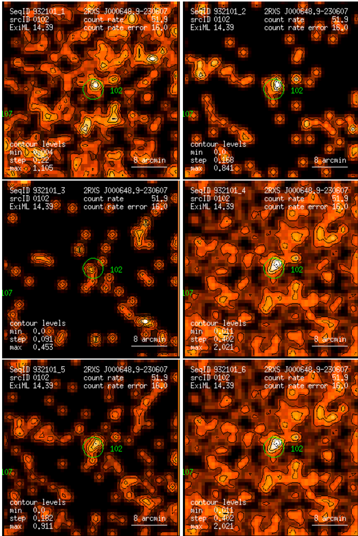
Figure 102: RASS 932101: detection 0102: band rate images, Gaussian filter: (1) PSPC channels 11 – 41, (2) 52 – 90, (3) 91 – 201, (4) 11 – 235, (5) 52 – 201, (6) 11 – 201. Broad band rates in counts/ks. Band rate contour levels in counts/ks/arcmin 2 .
