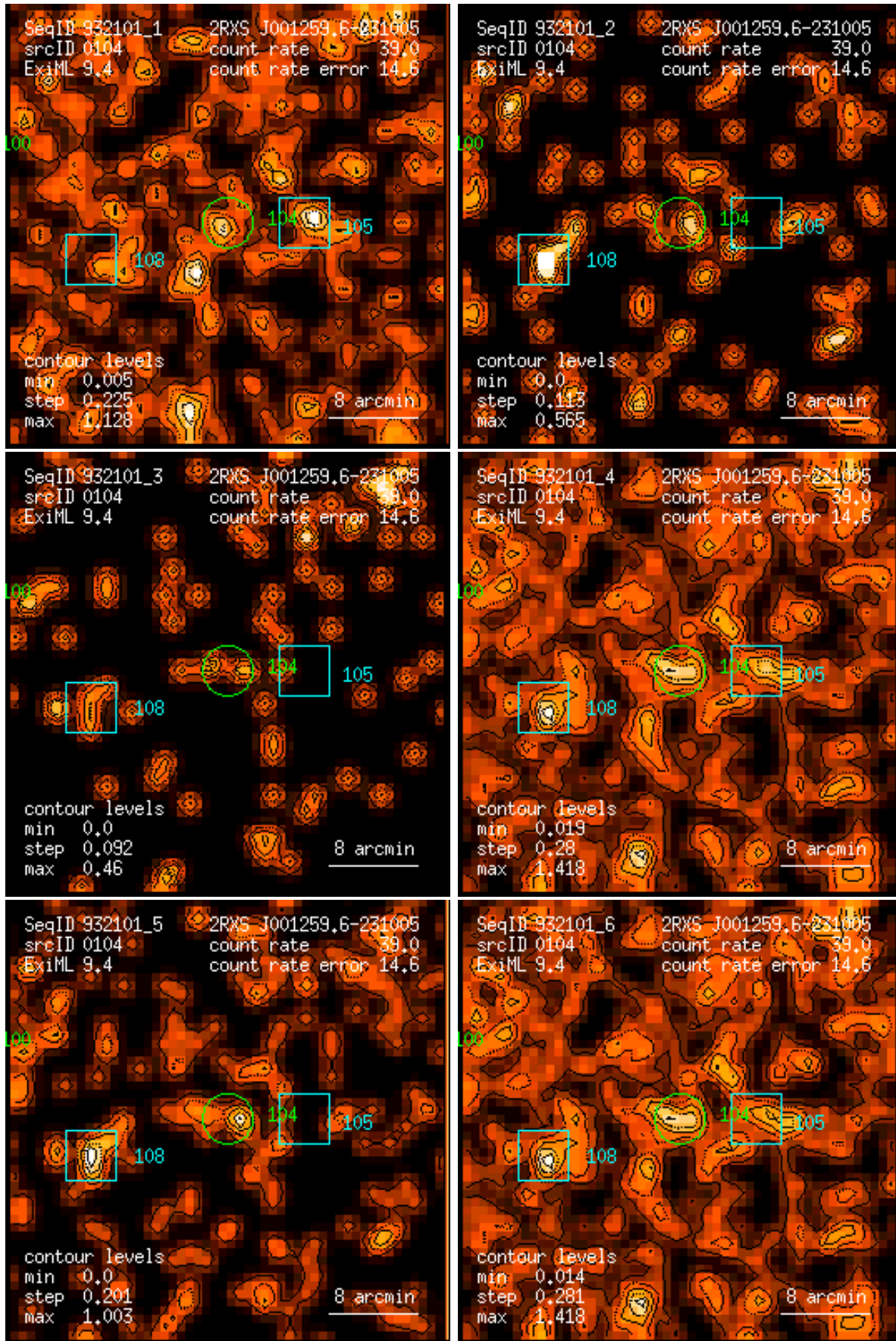
Figure 104: RASS 932101: detection 0104: band rate images, Gaussian filter: (1) PSPC channels 11 – 41, (2) 52 – 90, (3) 91 – 201, (4) 11 – 235, (5) 52 – 201, (6) 11 – 201. Broad band rates in counts/ks. Band rate contour levels in counts/ks/arcmin 2 .
