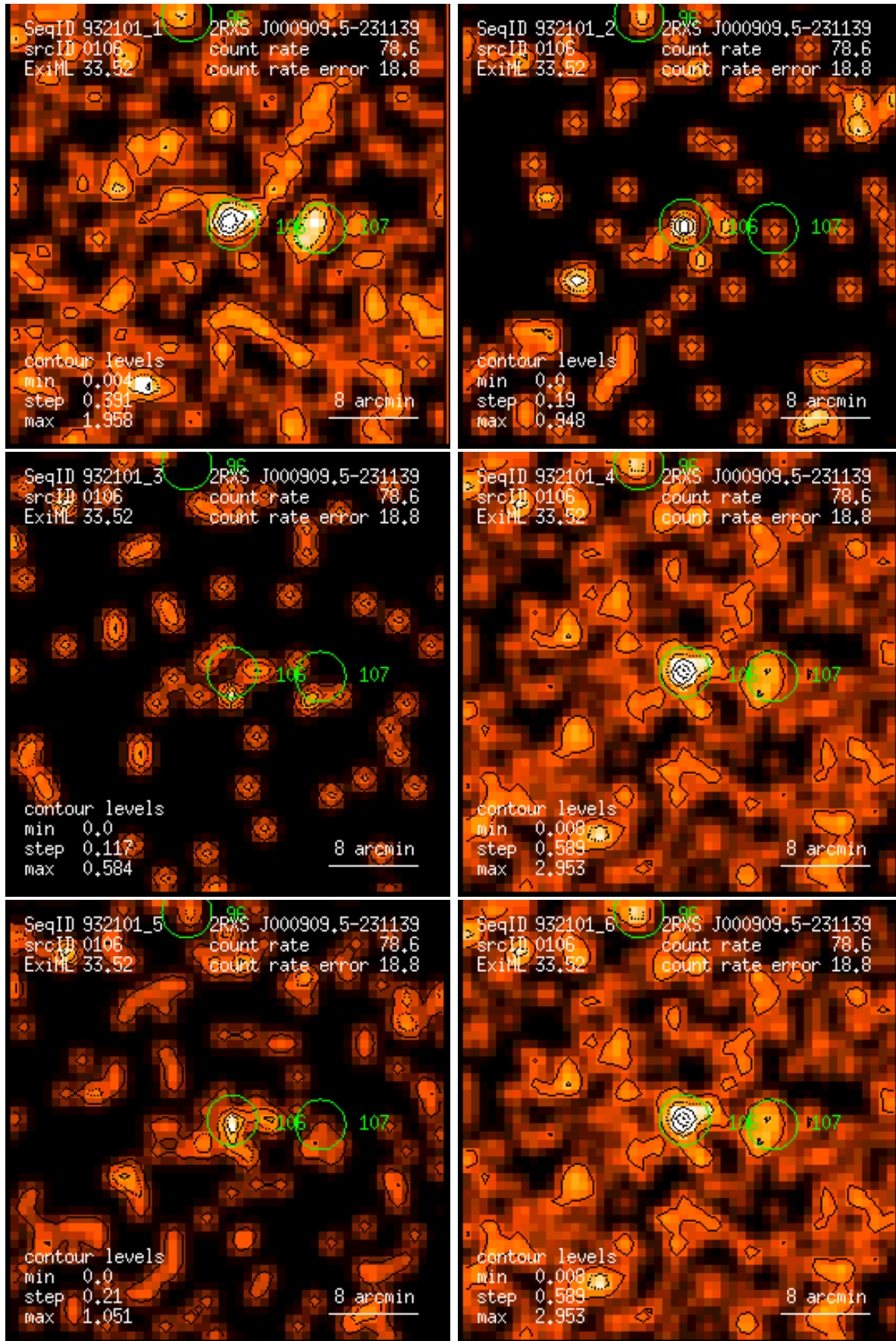
Figure 106: RASS 932101: detection 0106: band rate images, Gaussian filter: (1) PSPC channels 11 – 41, (2) 52 – 90, (3) 91 – 201, (4) 11 – 235, (5) 52 – 201, (6) 11 – 201. Broad band rates in counts/ks. Band rate contour levels in counts/ks/arcmin 2 .
