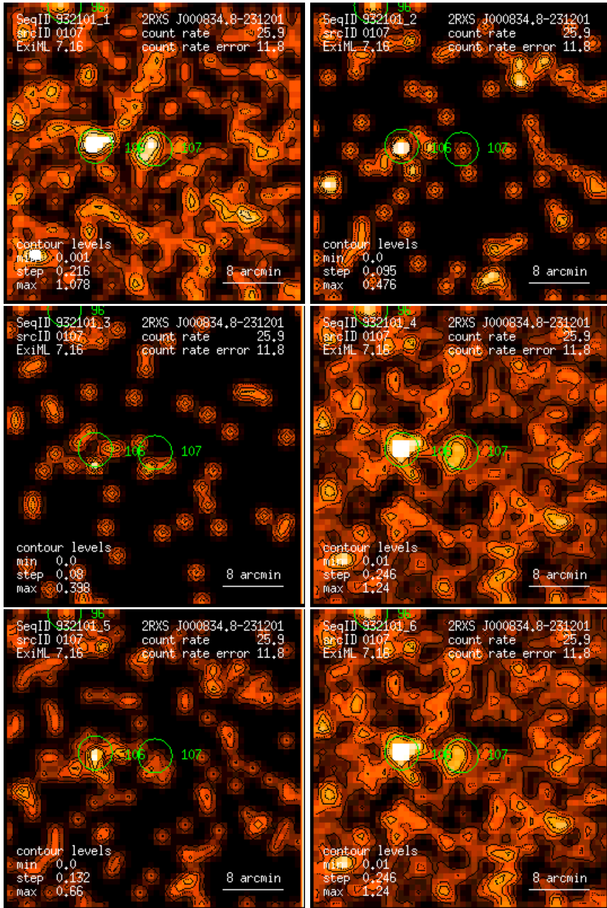
Figure 107: RASS 932101: detection 0107: band rate images, Gaussian filter: (1) PSPC channels 11 – 41, (2) 52 – 90, (3) 91 – 201, (4) 11 – 235, (5) 52 – 201, (6) 11 – 201. Broad band rates in counts/ks. Band rate contour levels in counts/ks/arcmin 2 .
