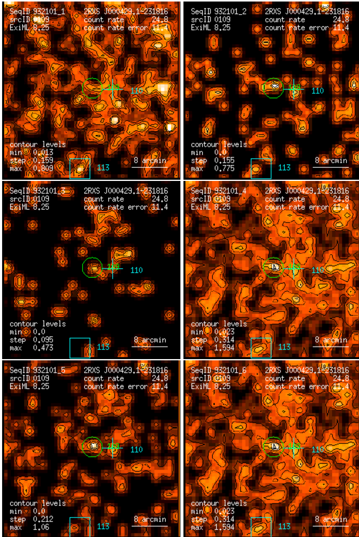
Figure 109: RASS 932101: detection 0109: band rate images, Gaussian filter: (1) PSPC channels 11 – 41, (2) 52 – 90, (3) 91 – 201, (4) 11 – 235, (5) 52 – 201, (6) 11 – 201. Broad band rates in counts/ks. Band rate contour levels in counts/ks/arcmin 2 .
