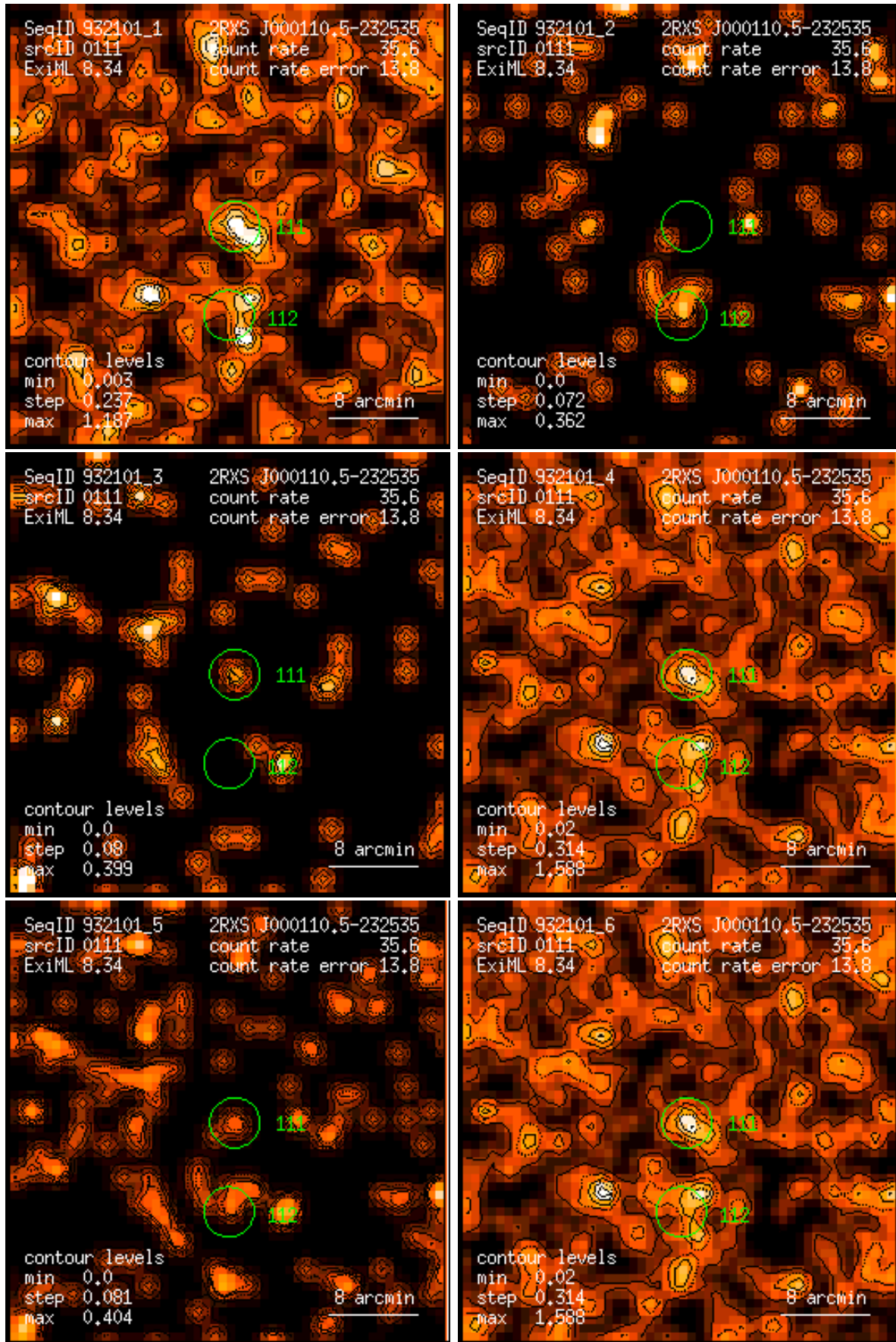
Figure 111: RASS 932101: detection 0111: band rate images, Gaussian filter: (1) PSPC channels 11 – 41, (2) 52 – 90, (3) 91 – 201, (4) 11 – 235, (5) 52 – 201, (6) 11 – 201. Broad band rates in counts/ks. Band rate contour levels in counts/ks/arcmin 2 .
