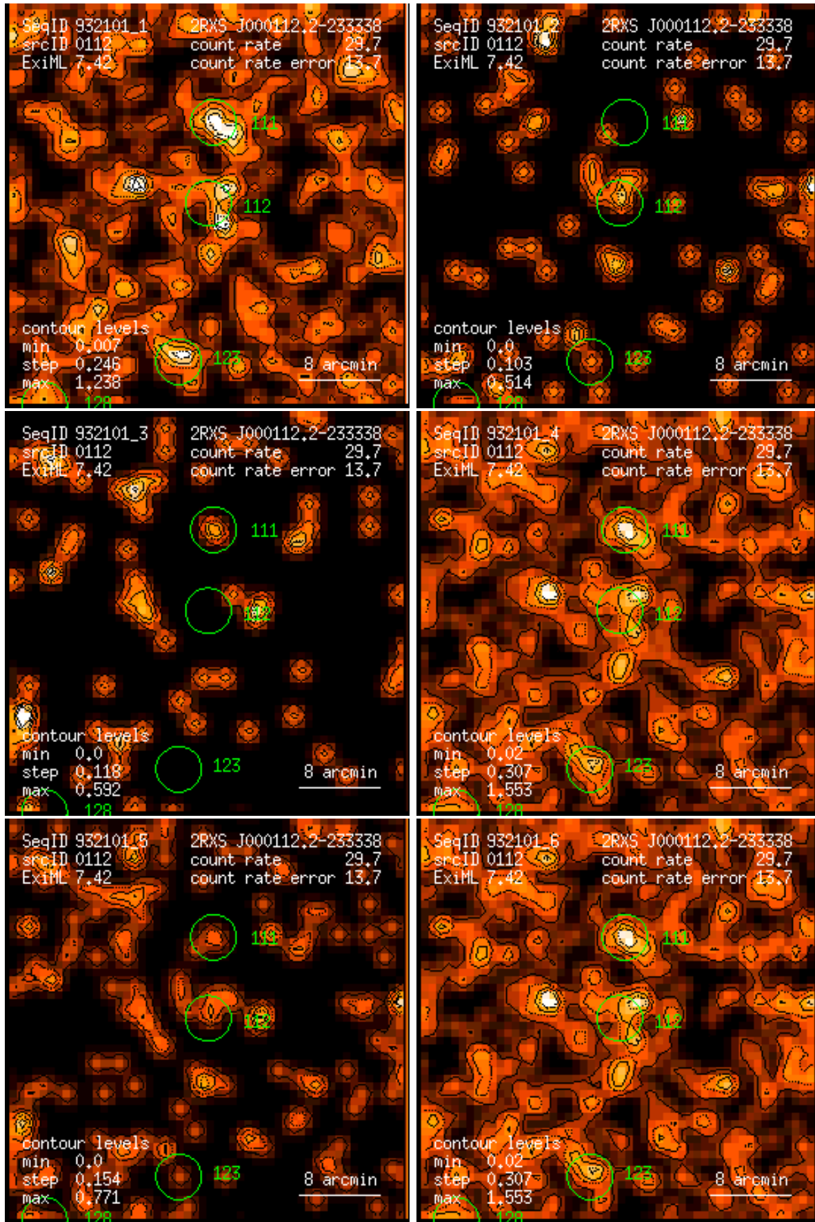
Figure 112: RASS 932101: detection 0112: band rate images, Gaussian filter: (1) PSPC channels 11 – 41, (2) 52 – 90, (3) 91 – 201, (4) 11 – 235, (5) 52 – 201, (6) 11 – 201. Broad band rates in counts/ks. Band rate contour levels in counts/ks/arcmin 2 .
