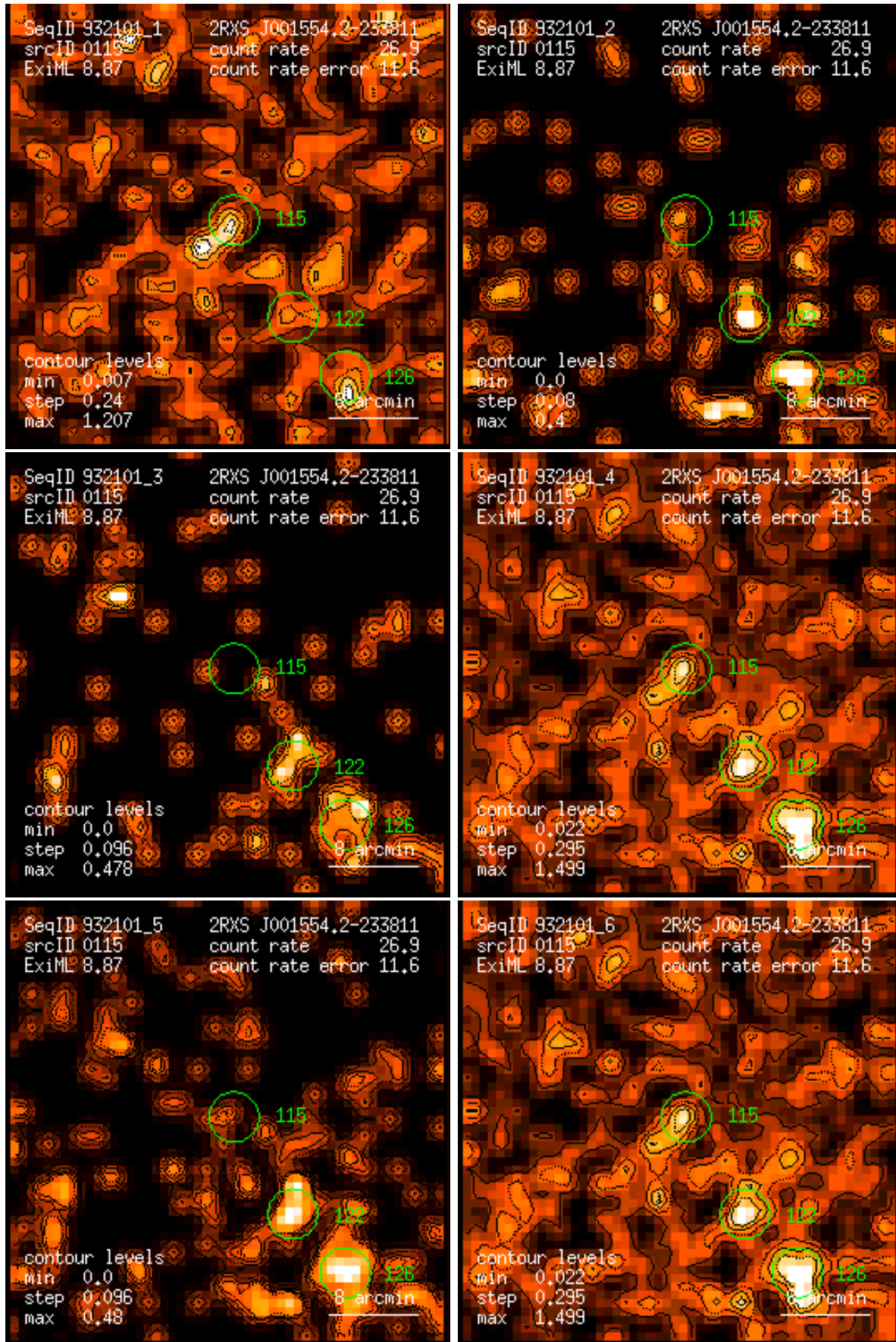
Figure 115: RASS 932101: detection 0115: band rate images, Gaussian filter: (1) PSPC channels 11 – 41, (2) 52 – 90, (3) 91 – 201, (4) 11 – 235, (5) 52 – 201, (6) 11 – 201. Broad band rates in counts/ks. Band rate contour levels in counts/ks/arcmin 2 .
