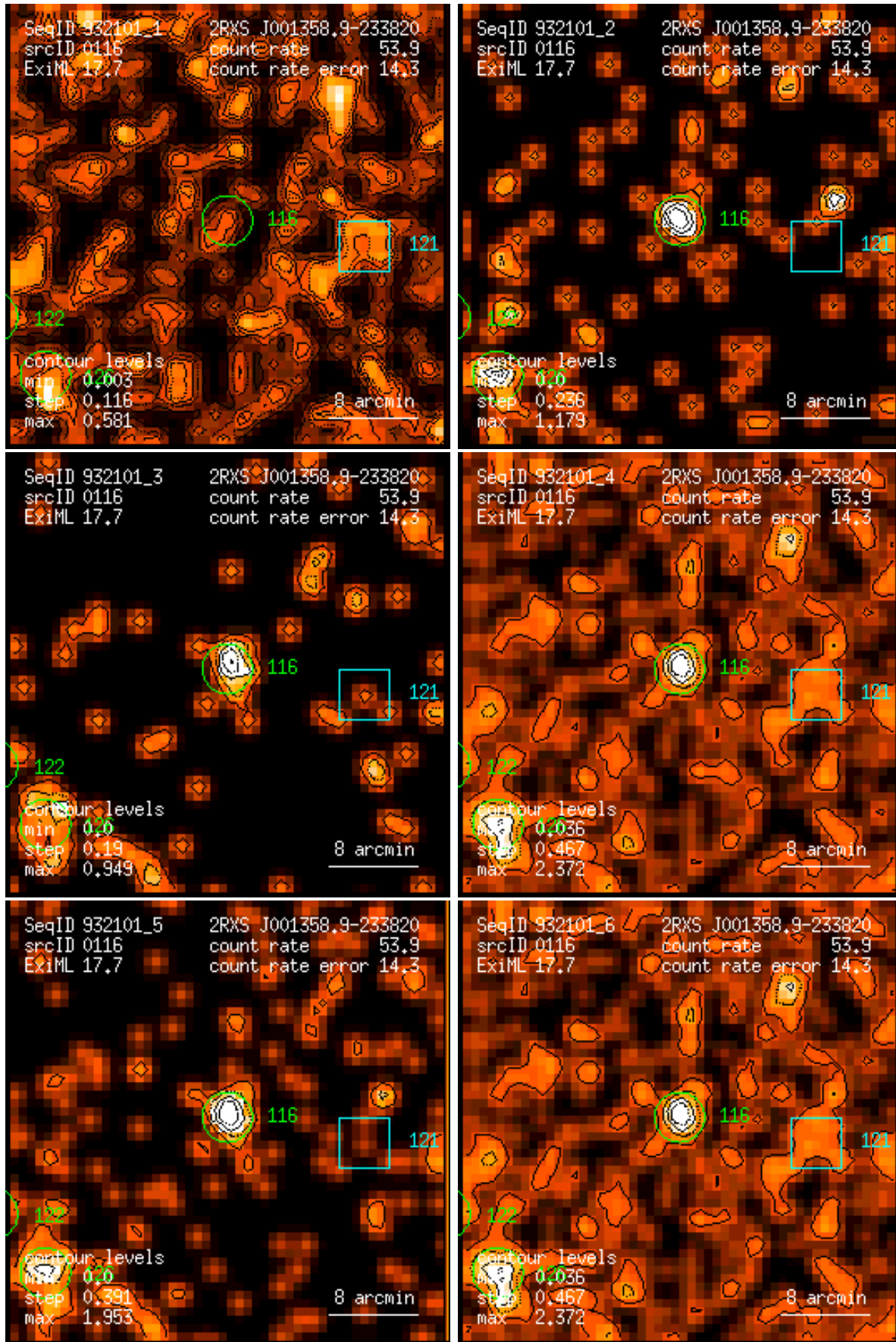
Figure 116: RASS 932101: detection 0116: band rate images, Gaussian filter: (1) PSPC channels 11 – 41, (2) 52 – 90, (3) 91 – 201, (4) 11 – 235, (5) 52 – 201, (6) 11 – 201. Broad band rates in counts/ks. Band rate contour levels in counts/ks/arcmin 2 .
