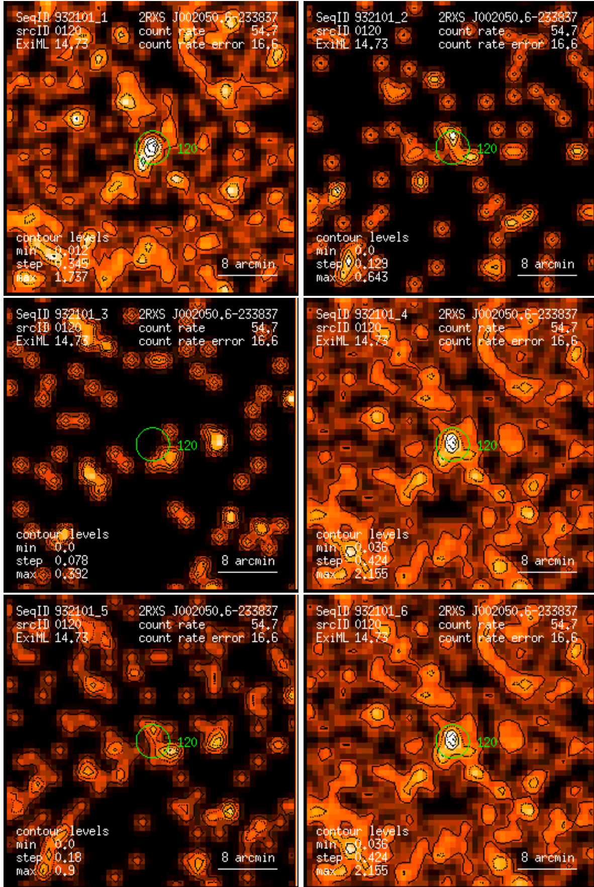
Figure 120: RASS 932101: detection 0120: band rate images, Gaussian filter: (1) PSPC channels 11 – 41, (2) 52 – 90, (3) 91 – 201, (4) 11 – 235, (5) 52 – 201, (6) 11 – 201. Broad band rates in counts/ks. Band rate contour levels in counts/ks/arcmin 2 .
