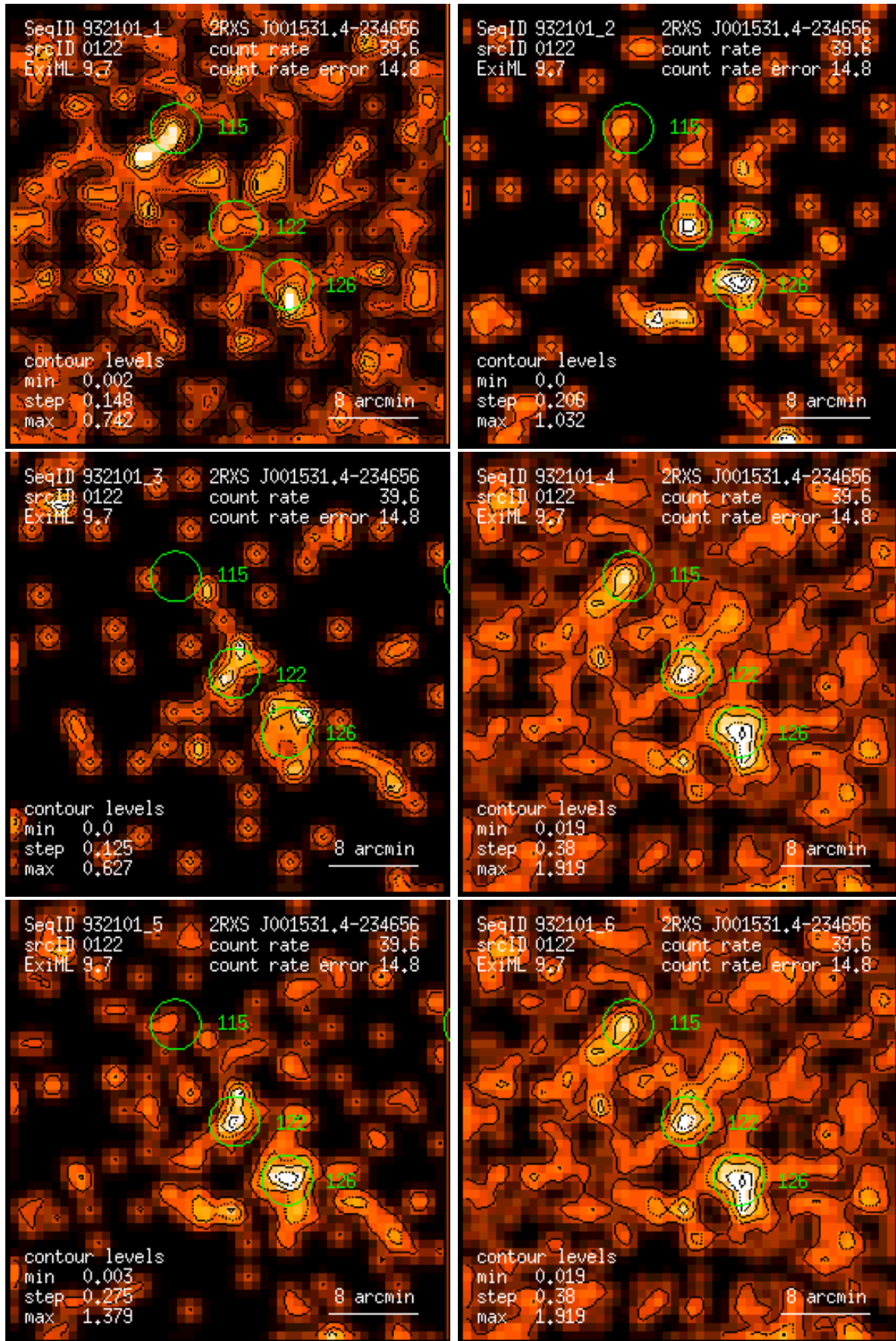
Figure 122: RASS 932101: detection 0122: band rate images, Gaussian filter: (1) PSPC channels 11 – 41, (2) 52 – 90, (3) 91 – 201, (4) 11 – 235, (5) 52 – 201, (6) 11 – 201. Broad band rates in counts/ks. Band rate contour levels in counts/ks/arcmin 2 .
