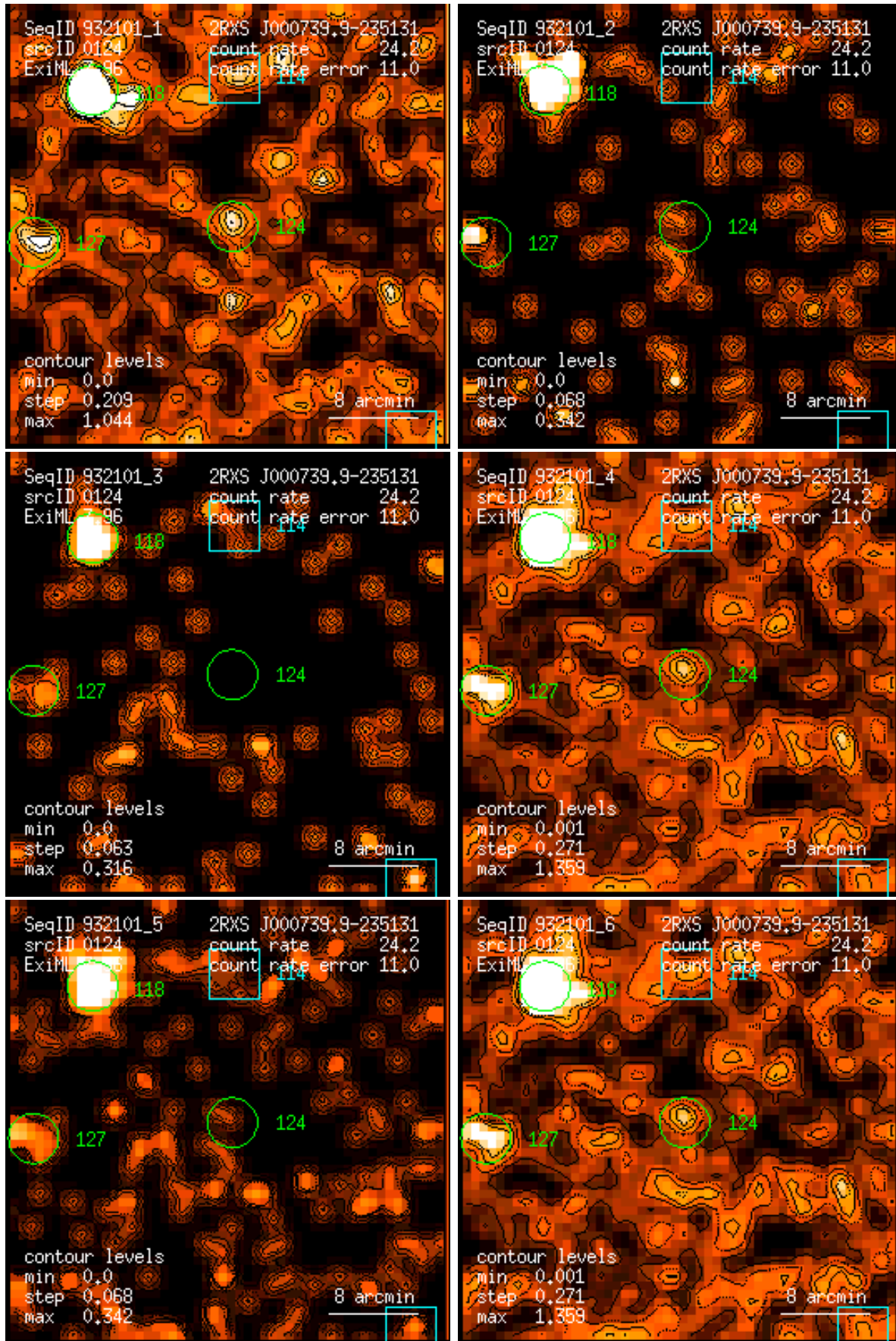
Figure 124: RASS 932101: detection 0124: band rate images, Gaussian filter: (1) PSPC channels 11 – 41, (2) 52 – 90, (3) 91 – 201, (4) 11 – 235, (5) 52 – 201, (6) 11 – 201. Broad band rates in counts/ks. Band rate contour levels in counts/ks/arcmin 2 .
